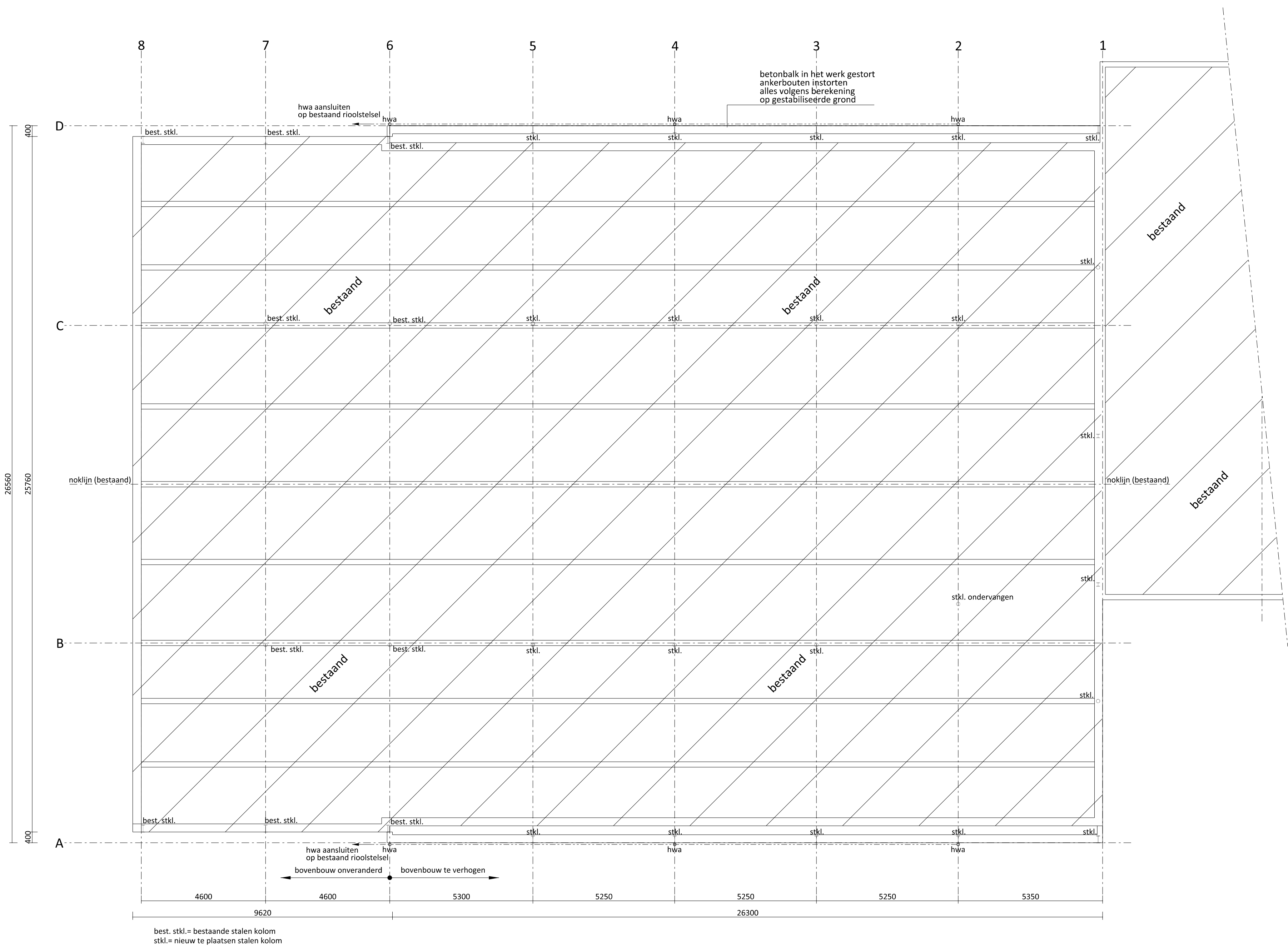
Funderingsplan
