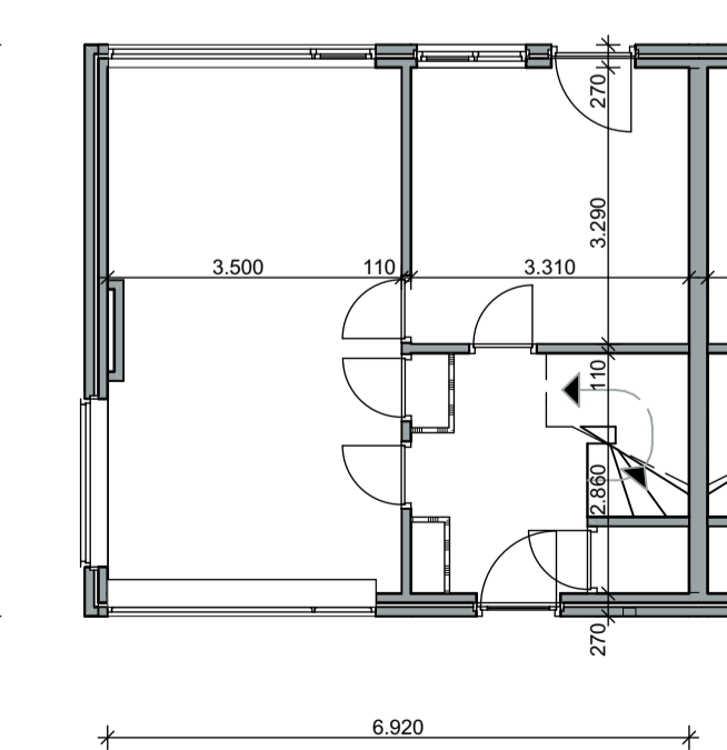
Begane grond 1/100
