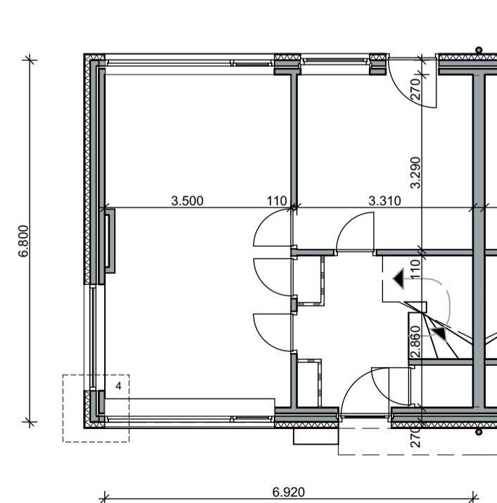
Begane grond 1/00
