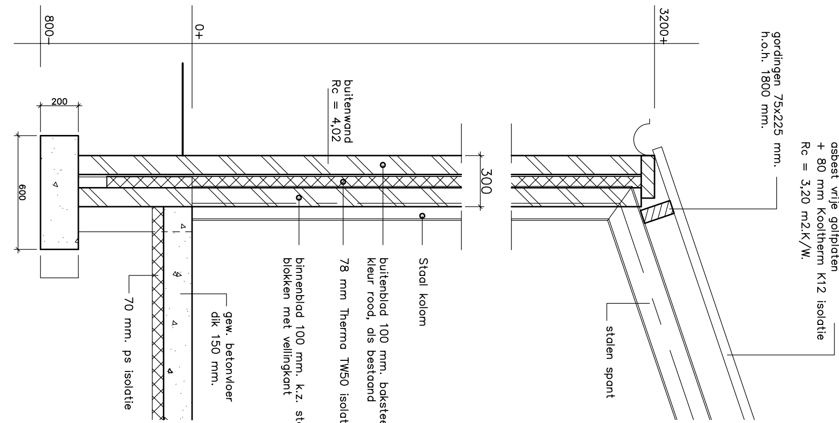
DETAIL 1
