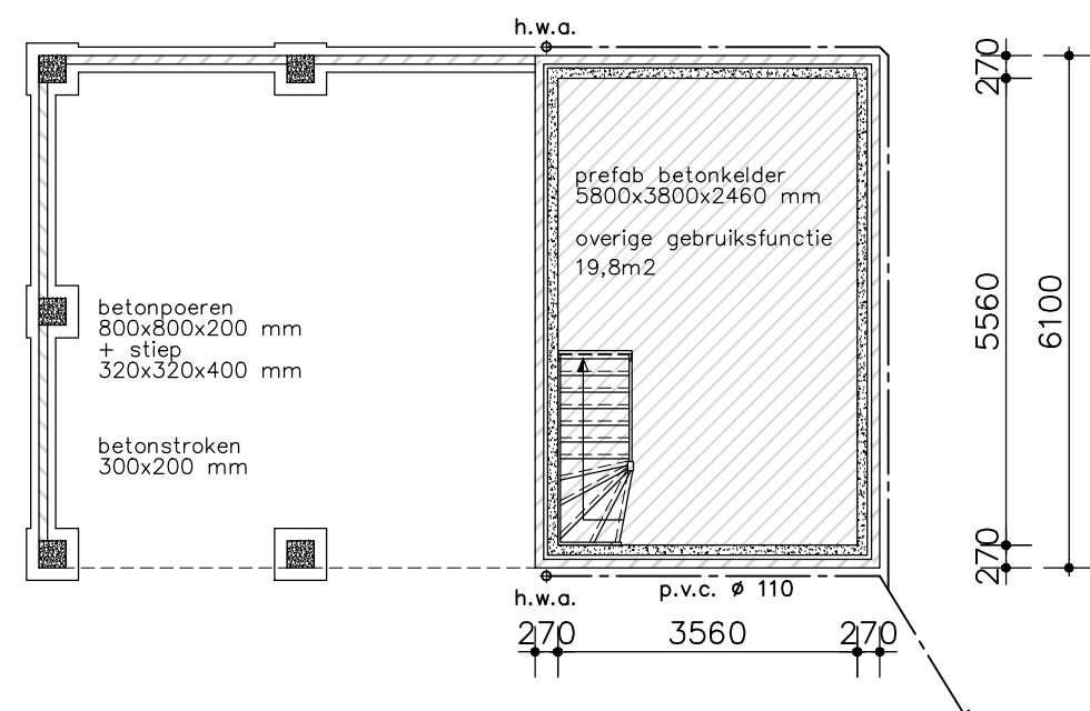
kelder/fundering
