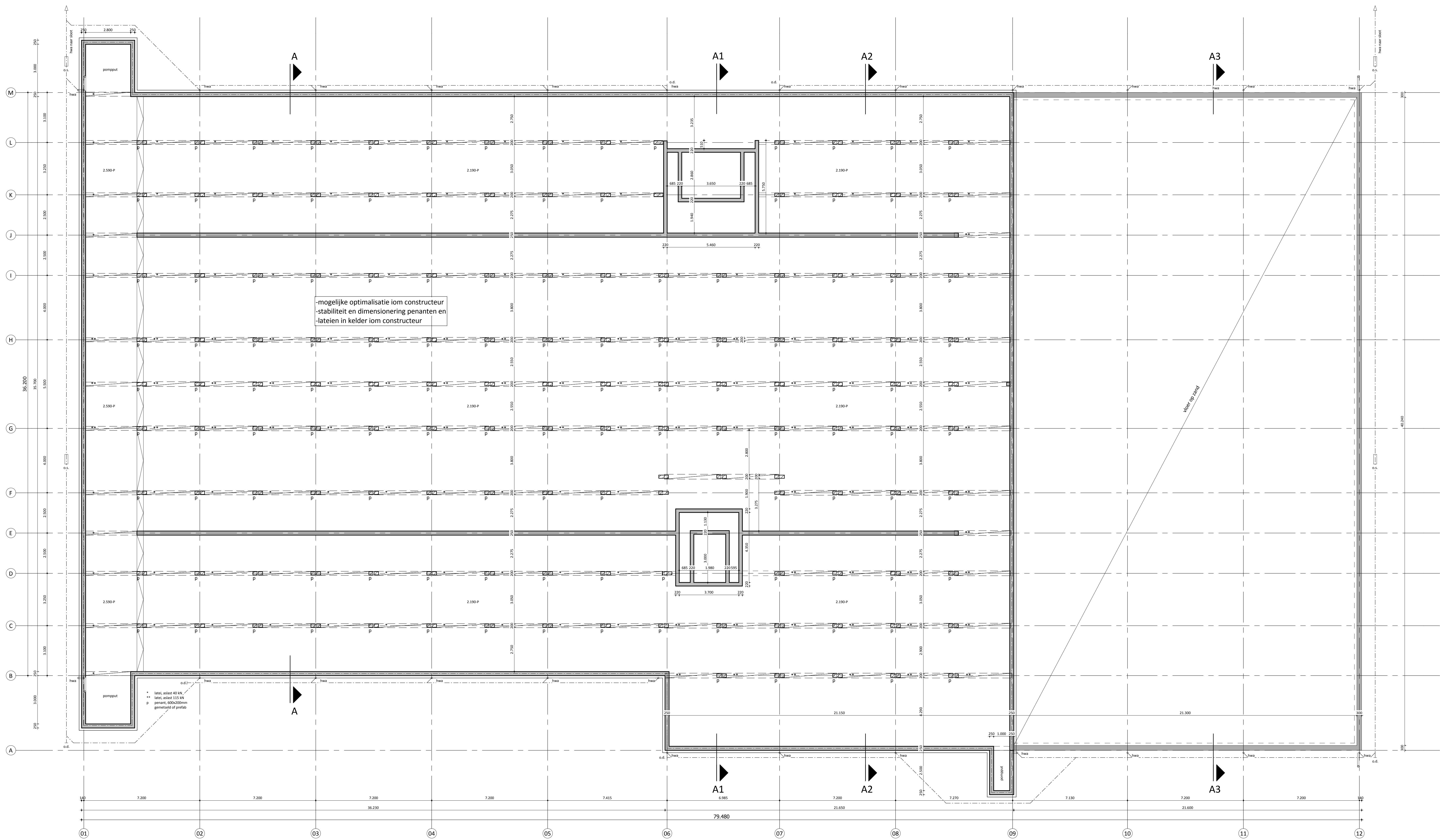
kelderplan
