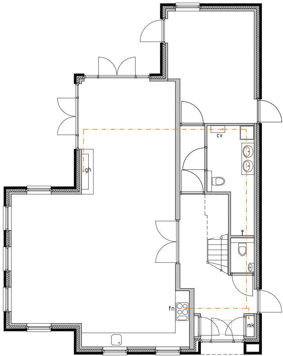
Gasinstallatie principe Begane grond
