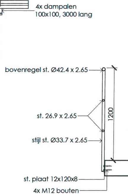
detail st. leuning 1:20
