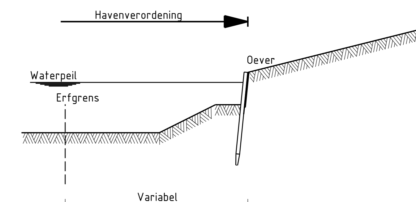
Principe detail Goese Meer
