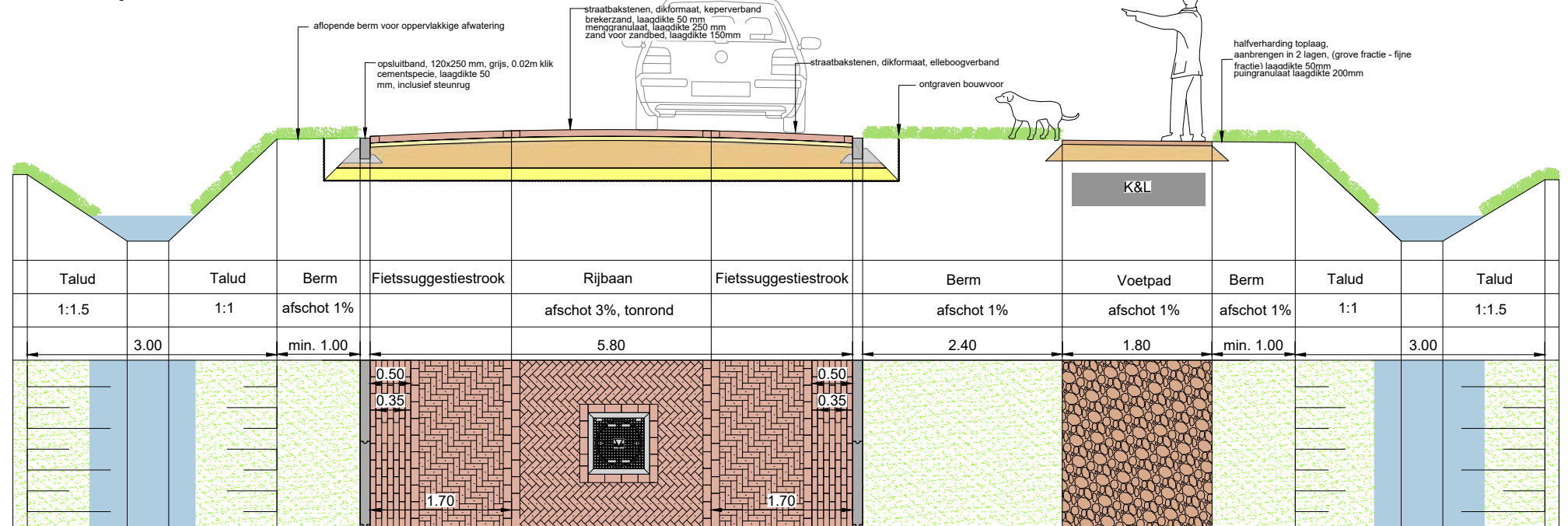
Profiel 10: Lint in groene mal
