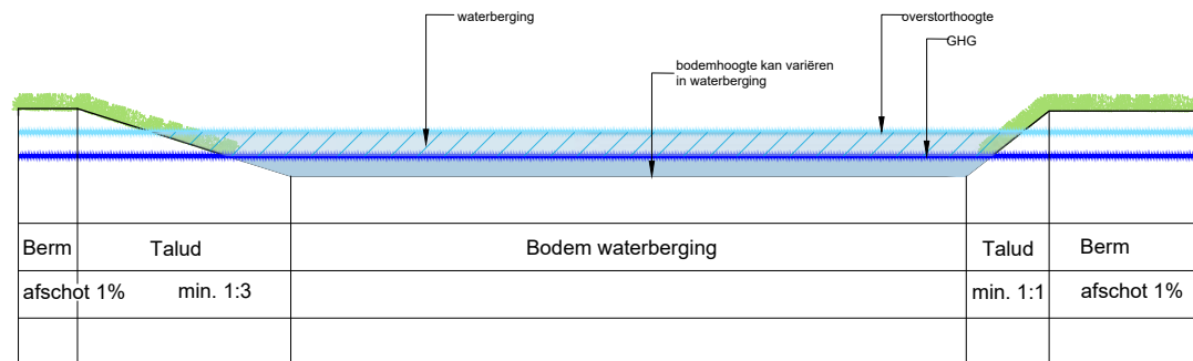
Profiel 11: Waterberging
