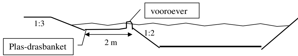
Figuur 1: profiel waterbergingsoever: plas-dras
