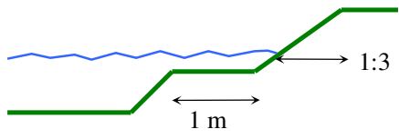
Figuur 1: profiel waterbergingsoever: plas-dras
