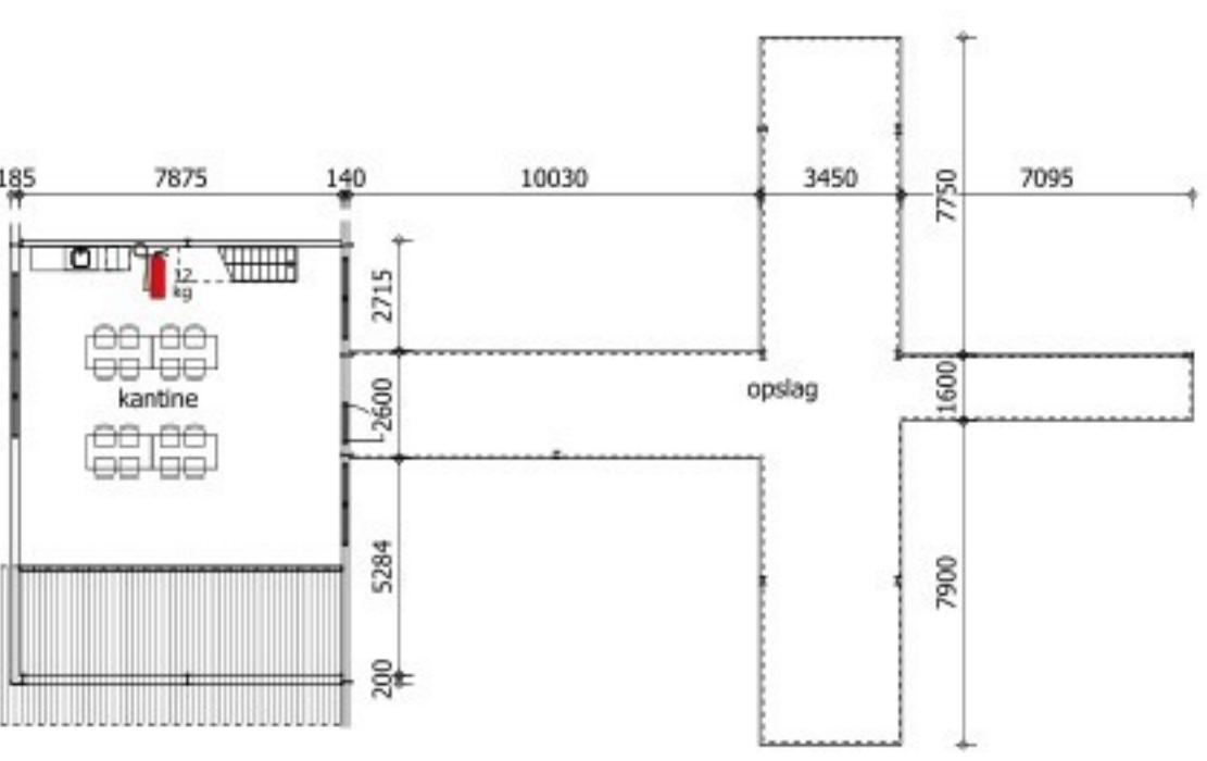
VERDIEPING STAL 9
