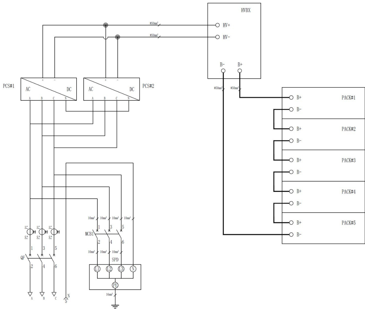
Figure 2-27 Circuit Diagram
