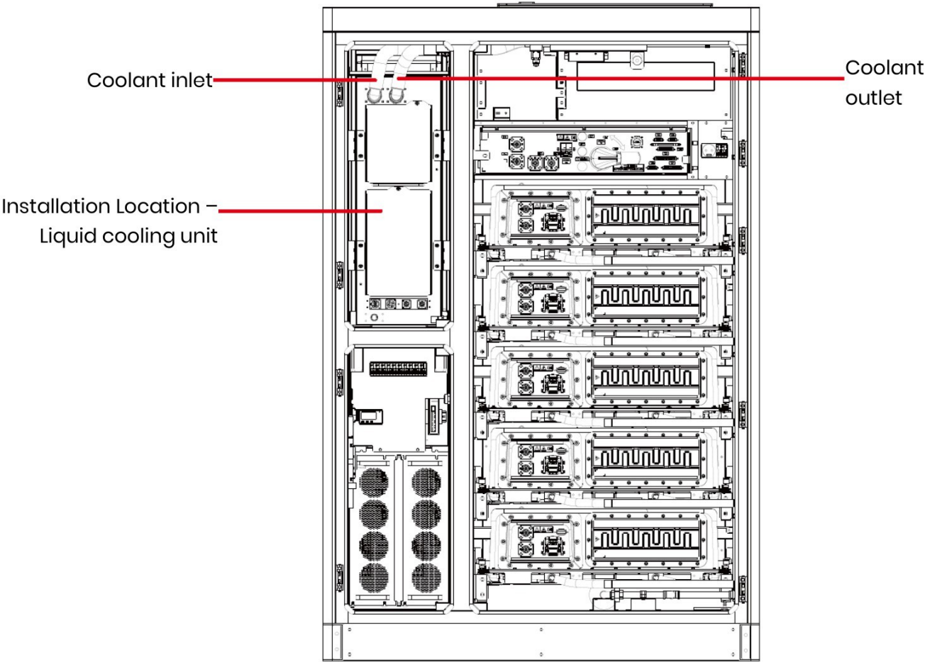
Figure 2-13 Liquid Cooling System Position
