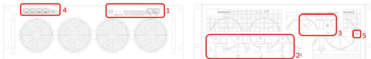
(1) Signal port (2) AC interface (3) DC interface (4) Paralleling interface (5) Grounding port
