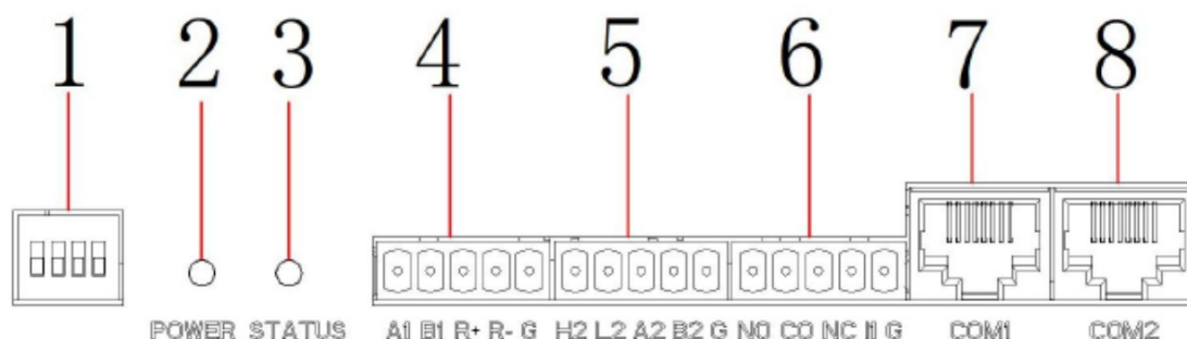
Figure 2-9 Signal Ports Schematic
