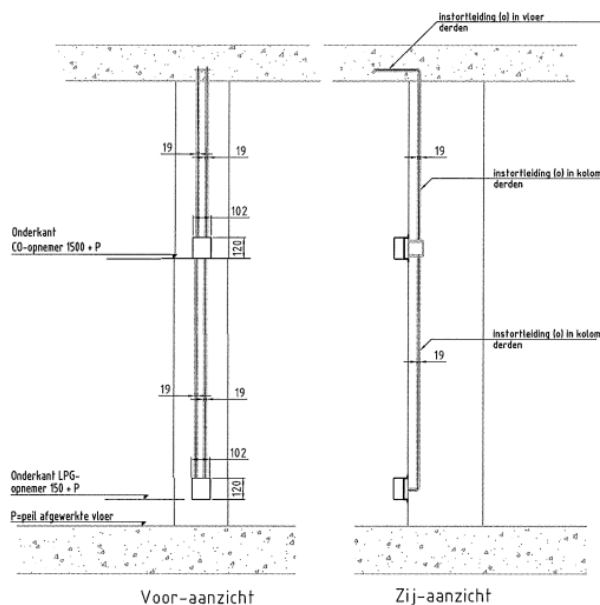
Principe-Detail CO/LPG Detectoren Instort / Schaal 1:20
