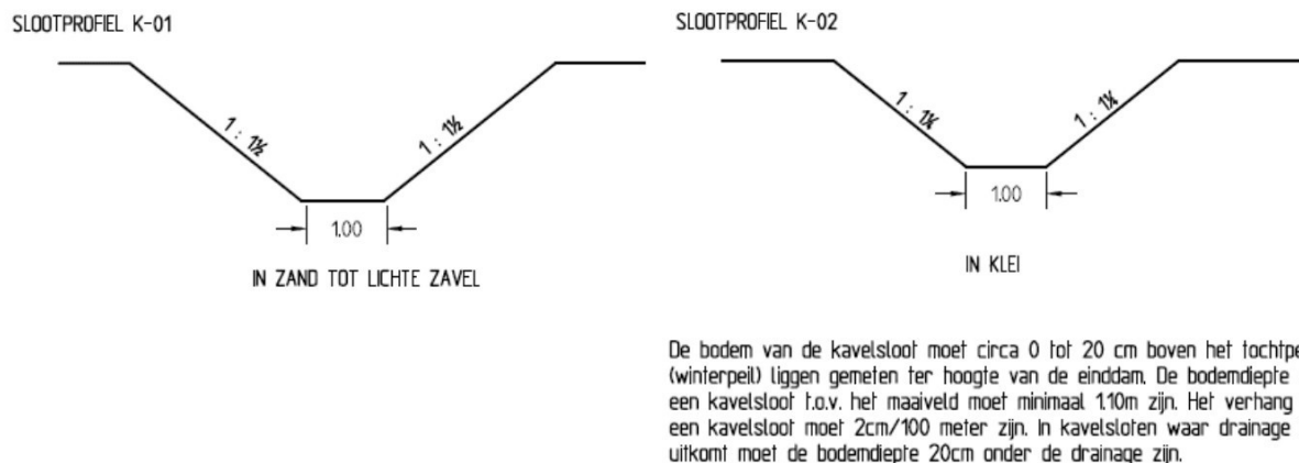
Figuur 6 – profiel kavelsloten (fragment leggetabel, blad 2)
