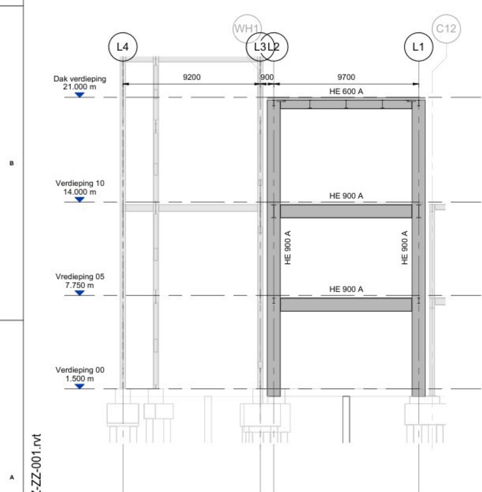
DOORSNEDE AS LC SCALE 1 : 150
