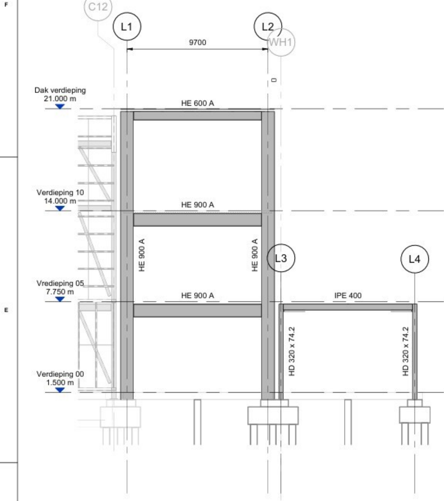
DOORSNEDE AS LA SCALE 1 : 150
