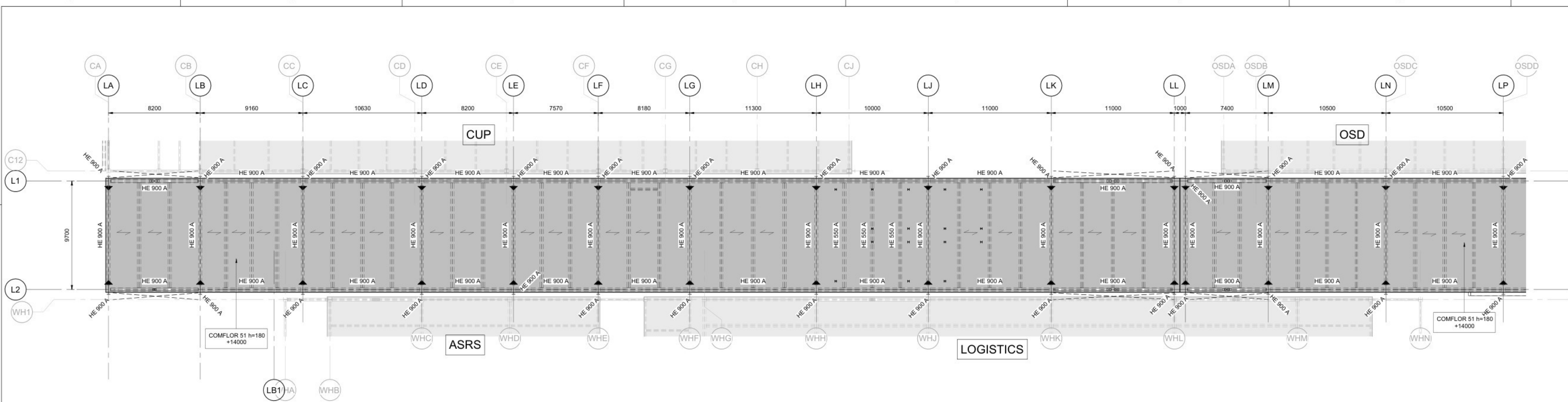
LEVEL 10 PLAN OVERALL - PRE-PERMITTING - ZONE A SCALE 1 : 150
