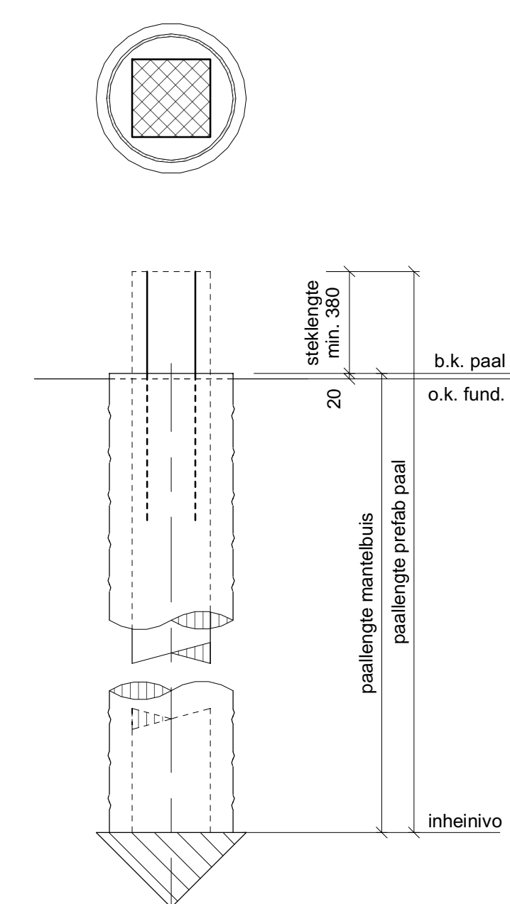
Alg. detail Fundex combi paal
