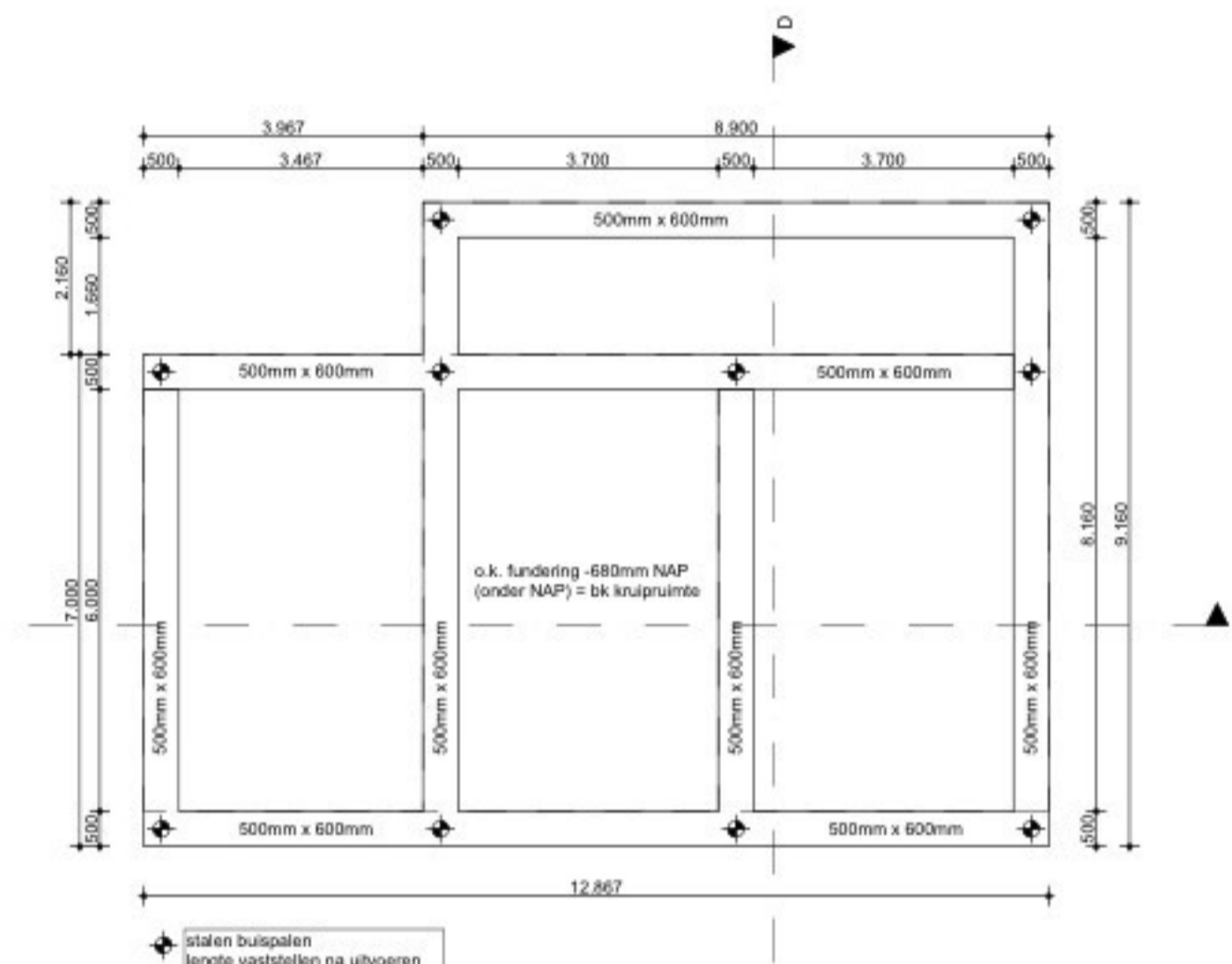
Fundering
