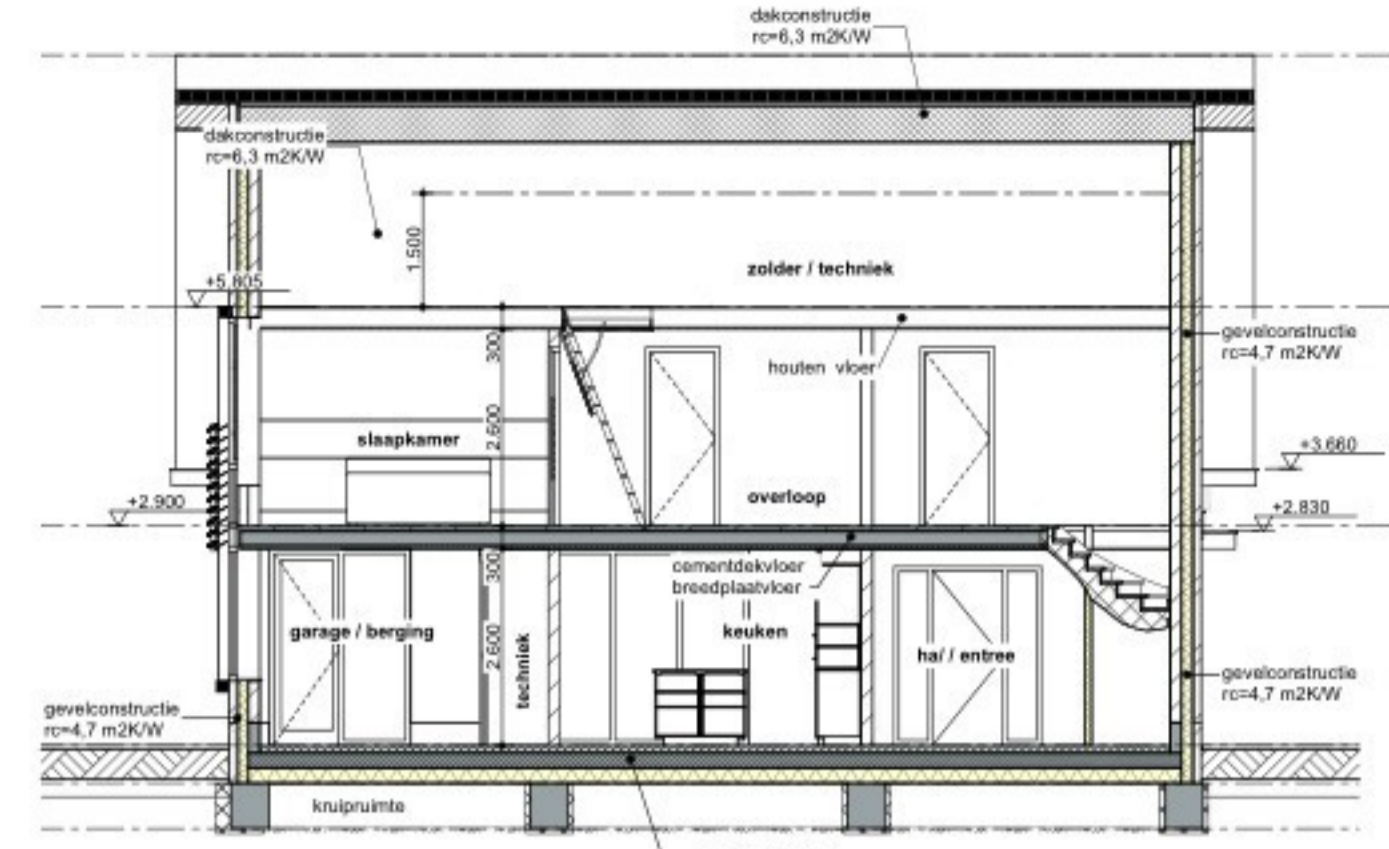
langdoorsnede (L)
