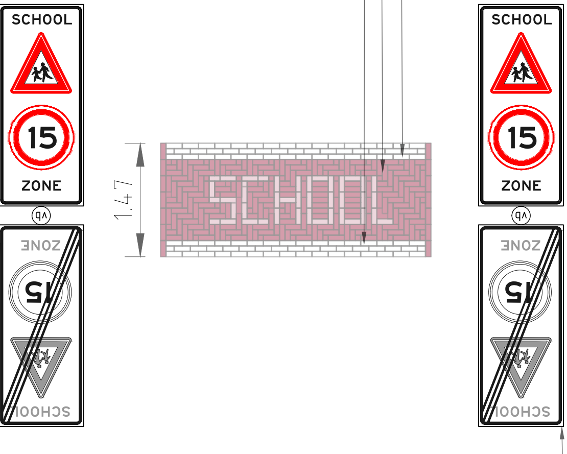
Detail schoolzone (1:50): SBS dikformaat
