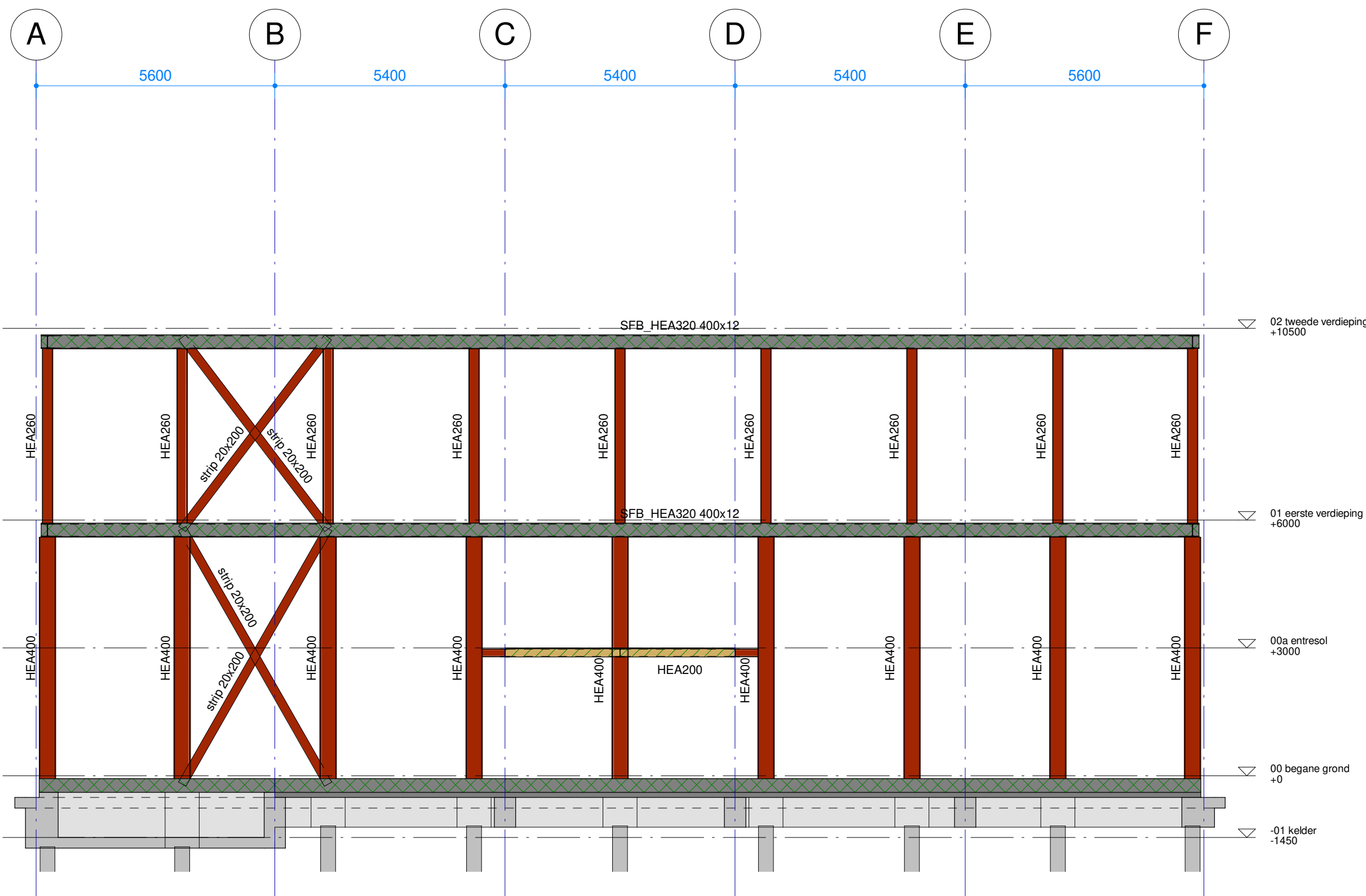
Doorsnede as 1 Schaal: 1 : 100
