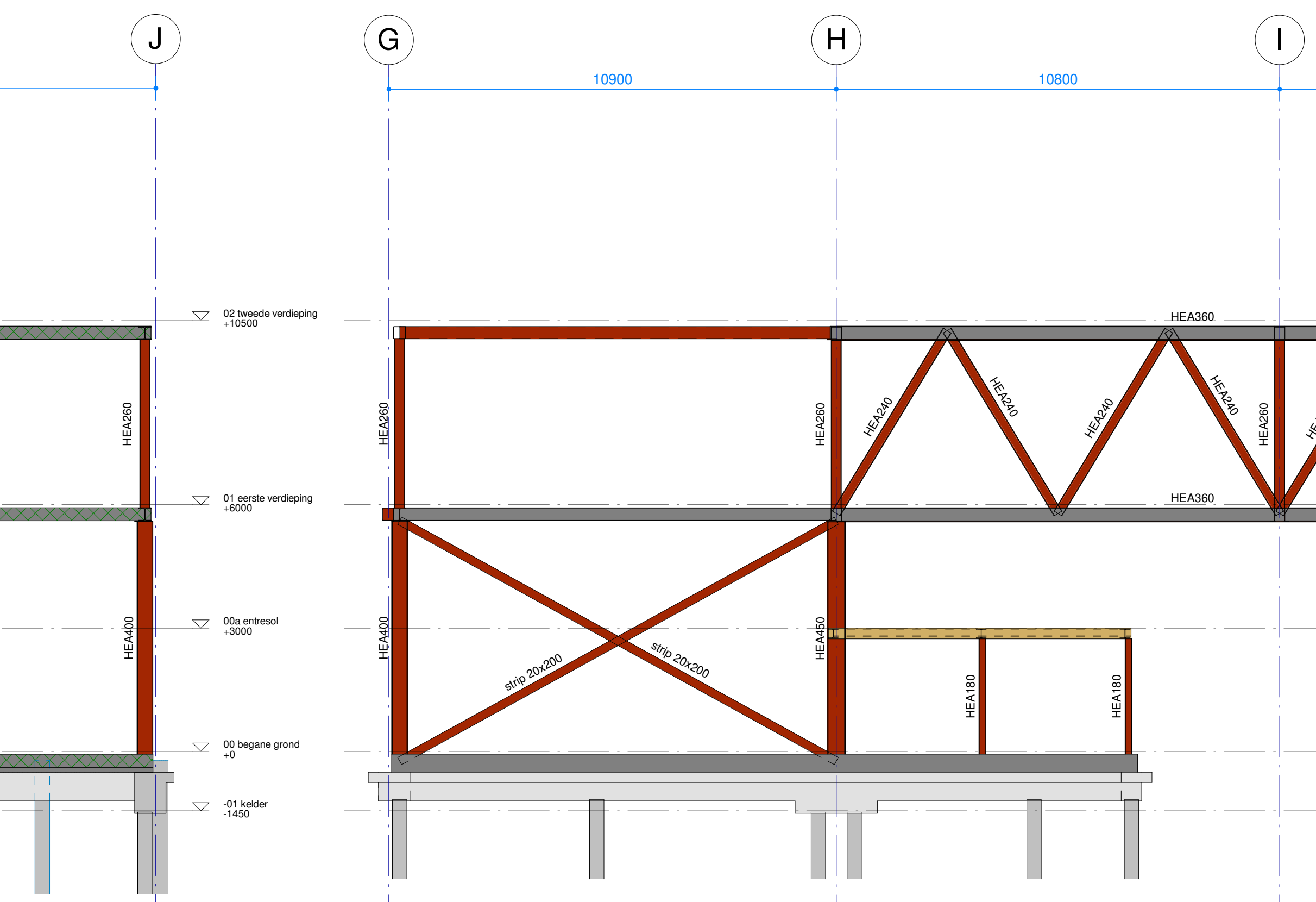
Doorsnede as 21 Schaal: 1 : 100
