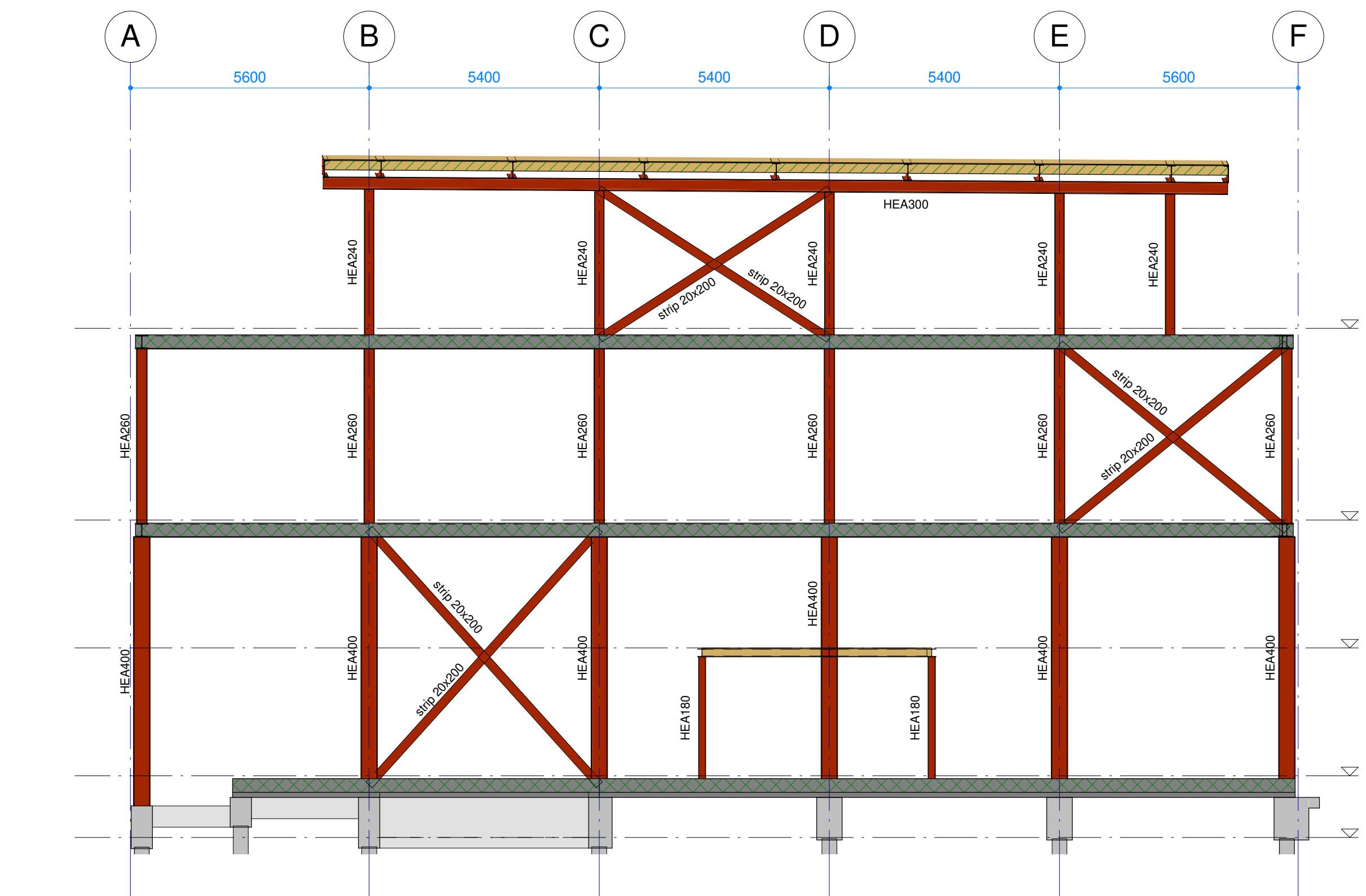
Doorsnede as 8 Schaal: 1 : 100
