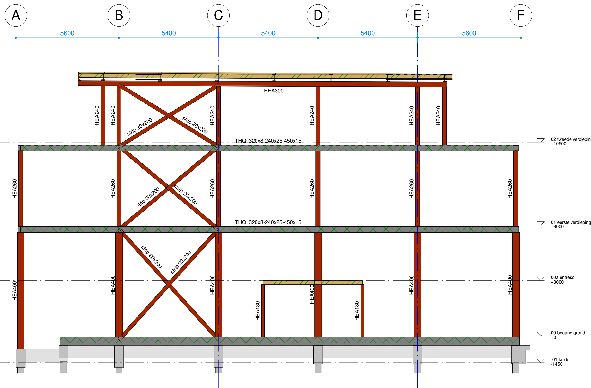
Doorsnede as 6 Schaal: 1 : 100
