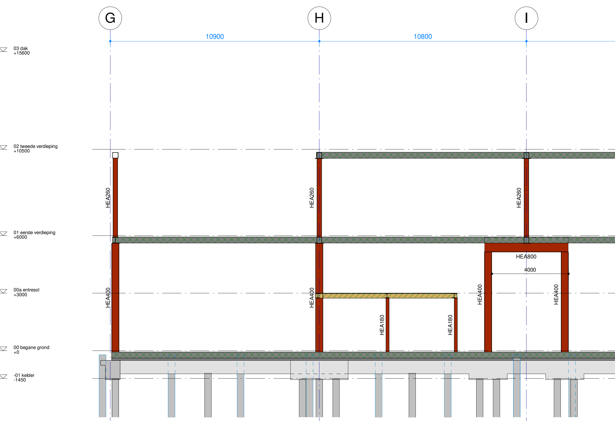
Doorsnede as 20 Schaal: 1 : 100
