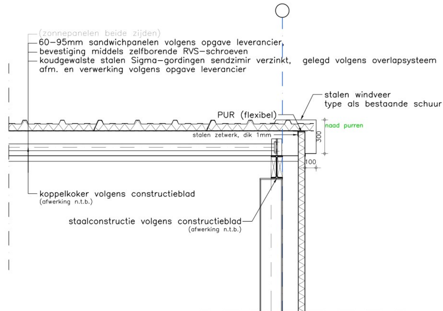
Detail windveer
