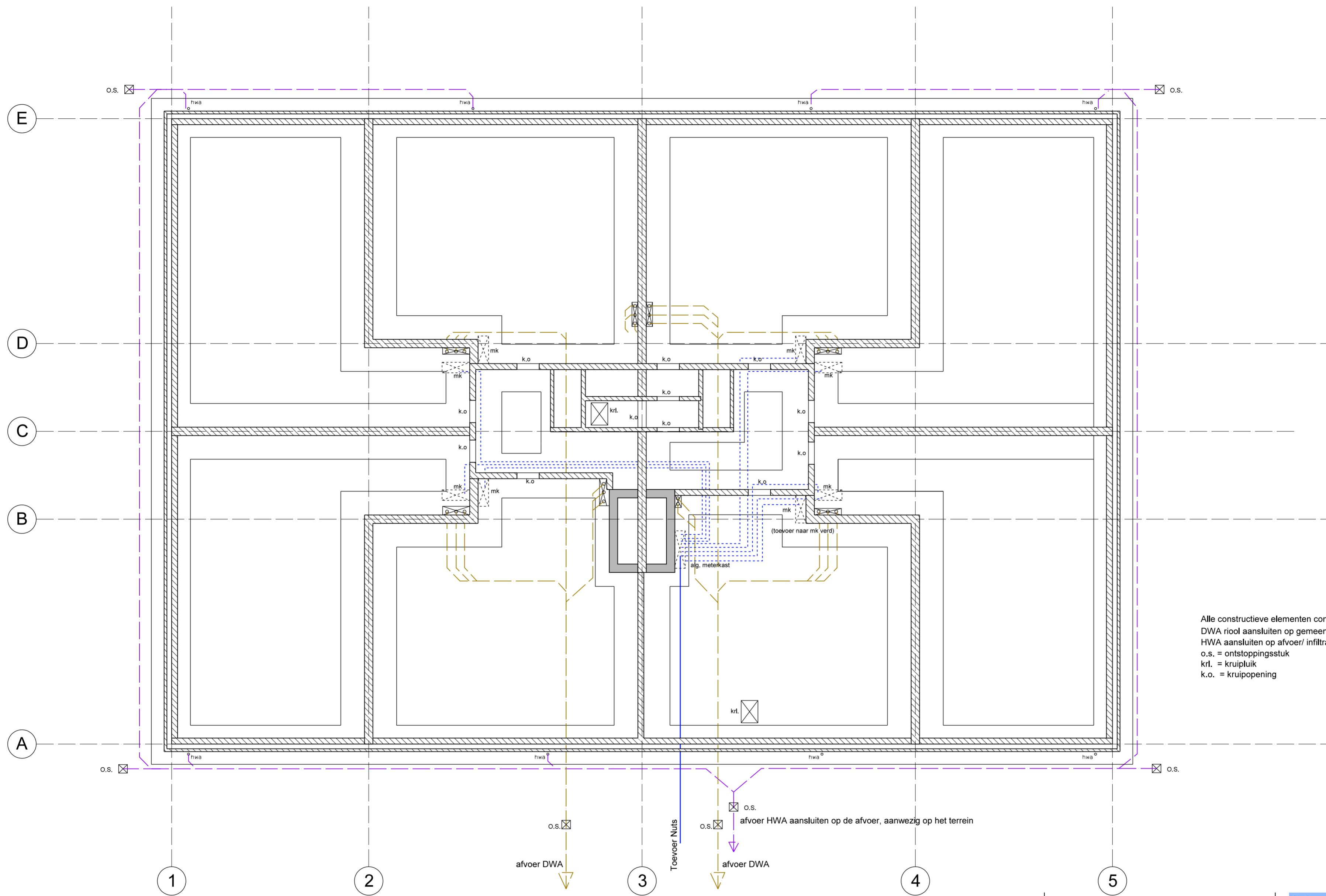
rioleringsplan
