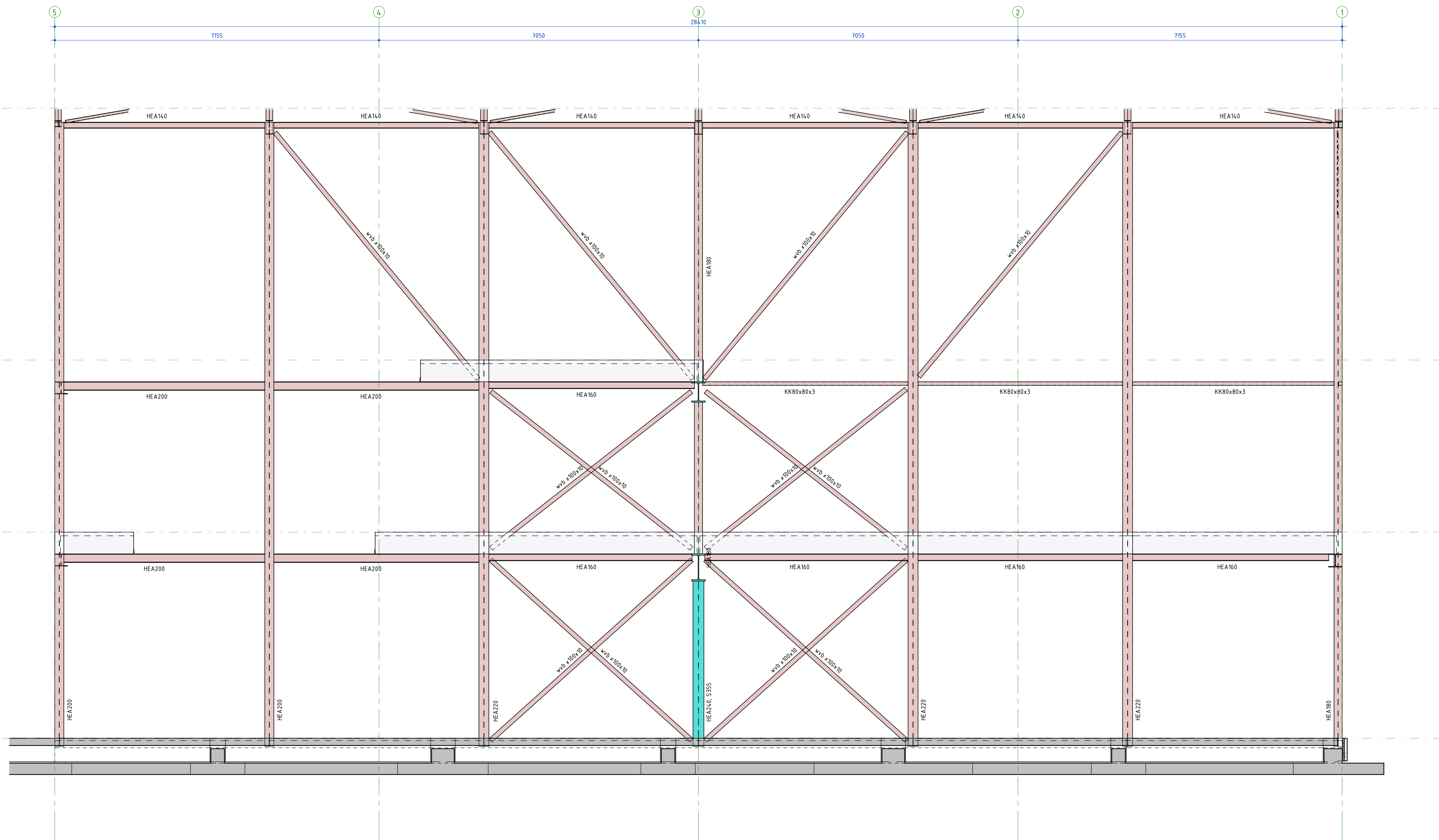
Aanzicht As A
