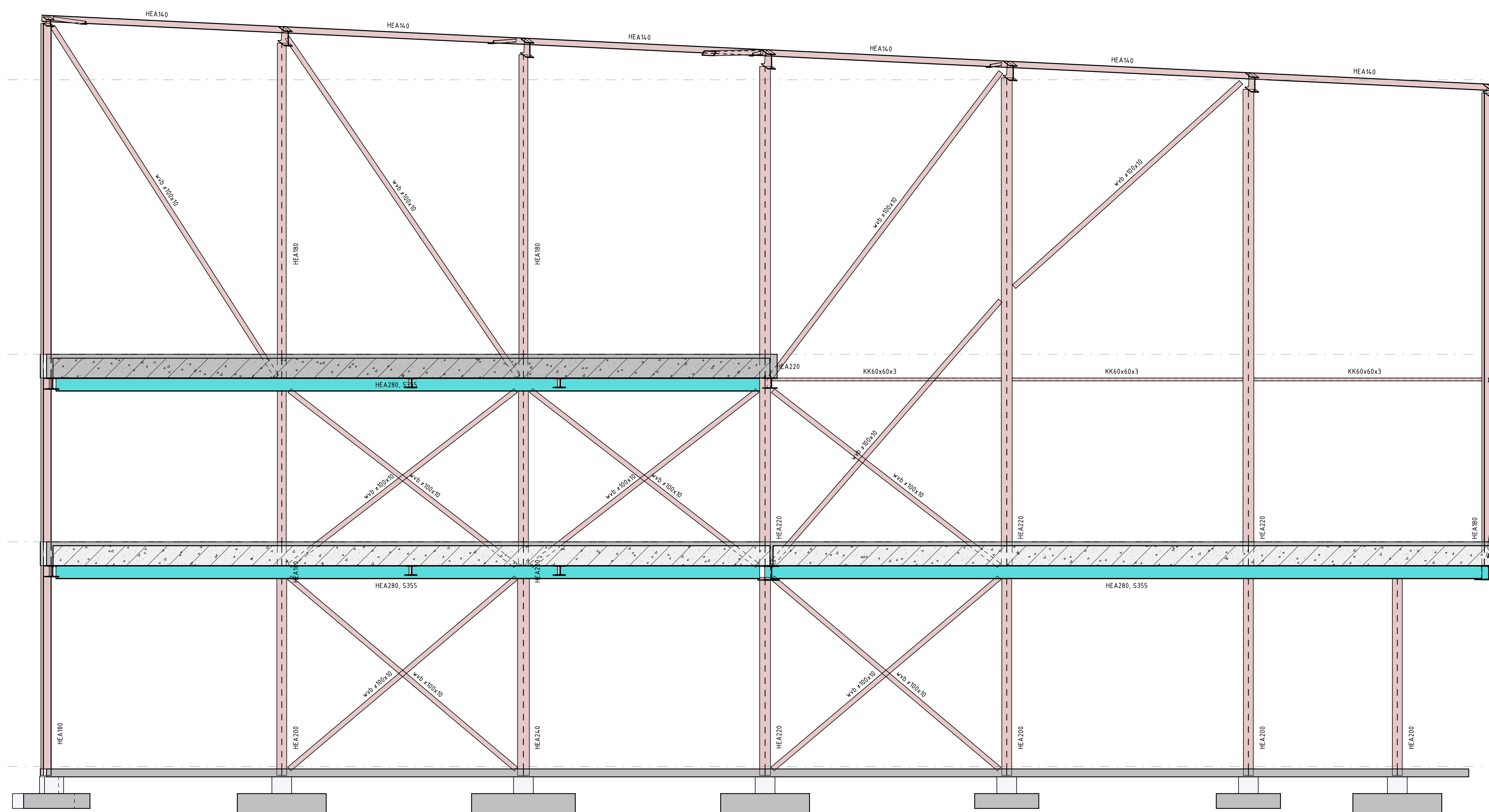
Aanzicht As A
