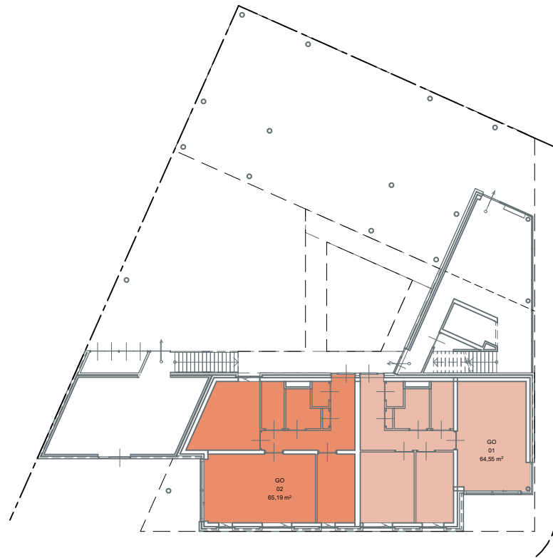
00 begane grond
