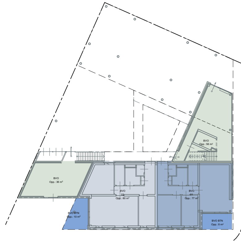
00 begane grond
