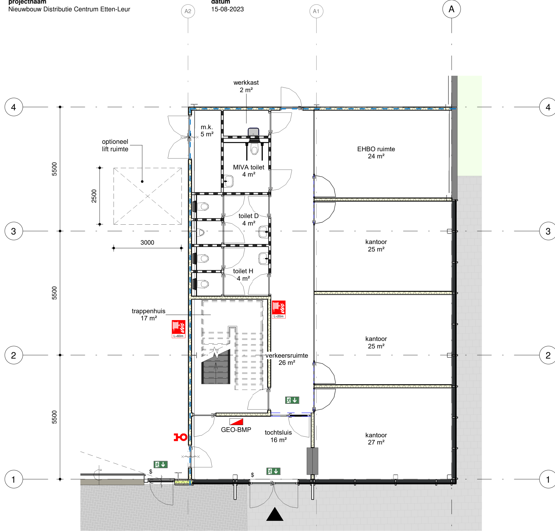
begane grond (Peil = 0)
