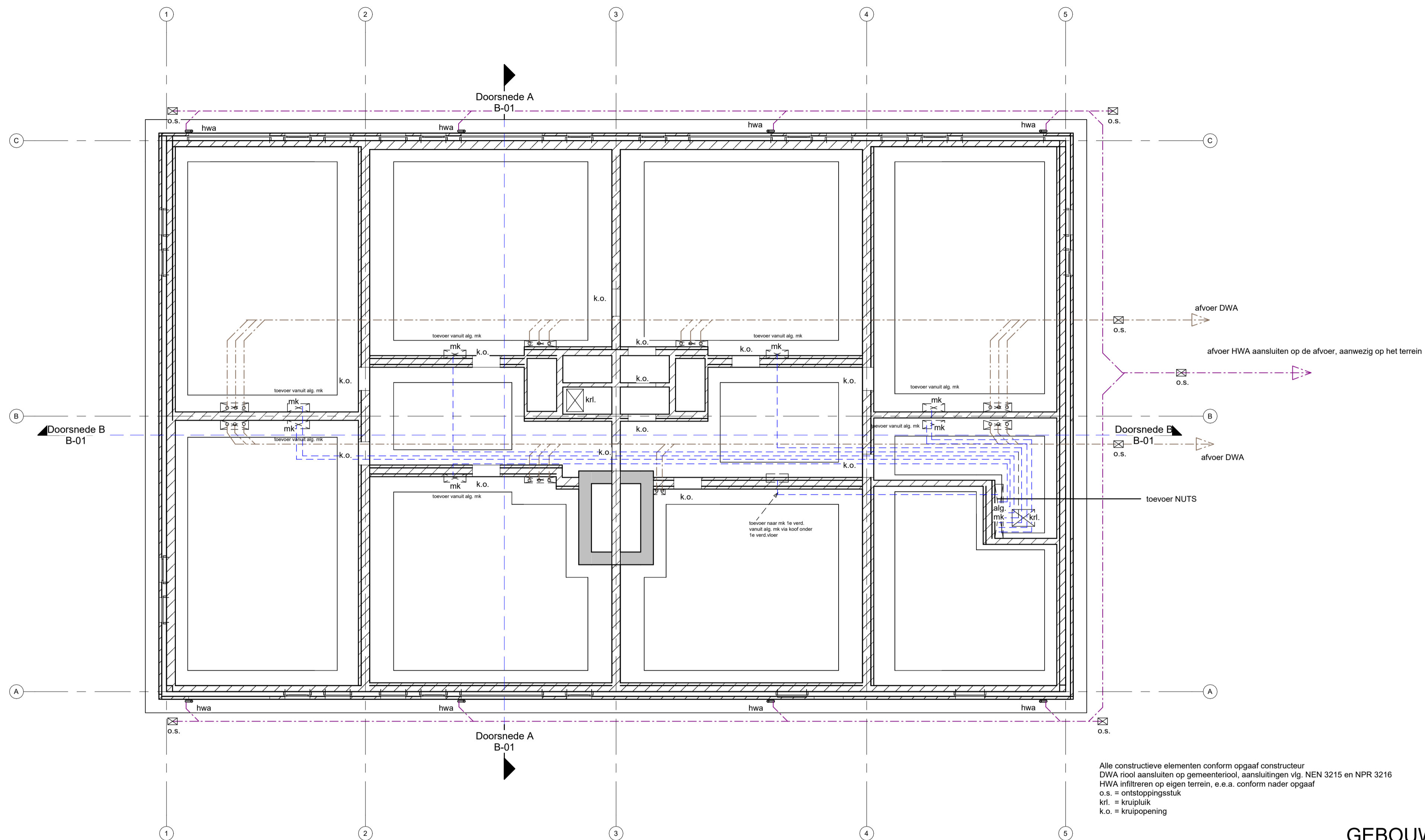
Rioleringsplan
