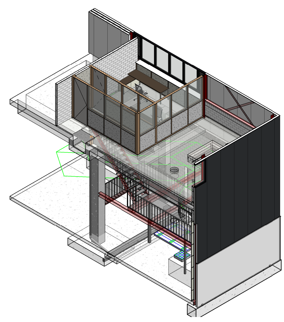
3D isometrie - trap pulper
