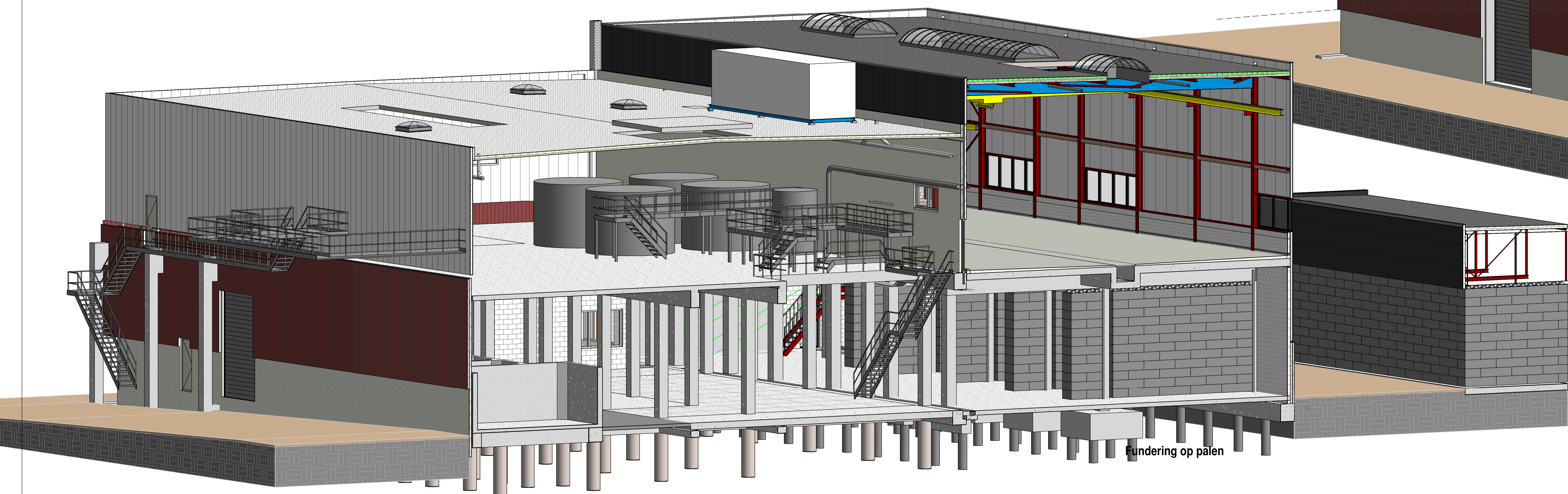
3D dwarsdoorsnede
