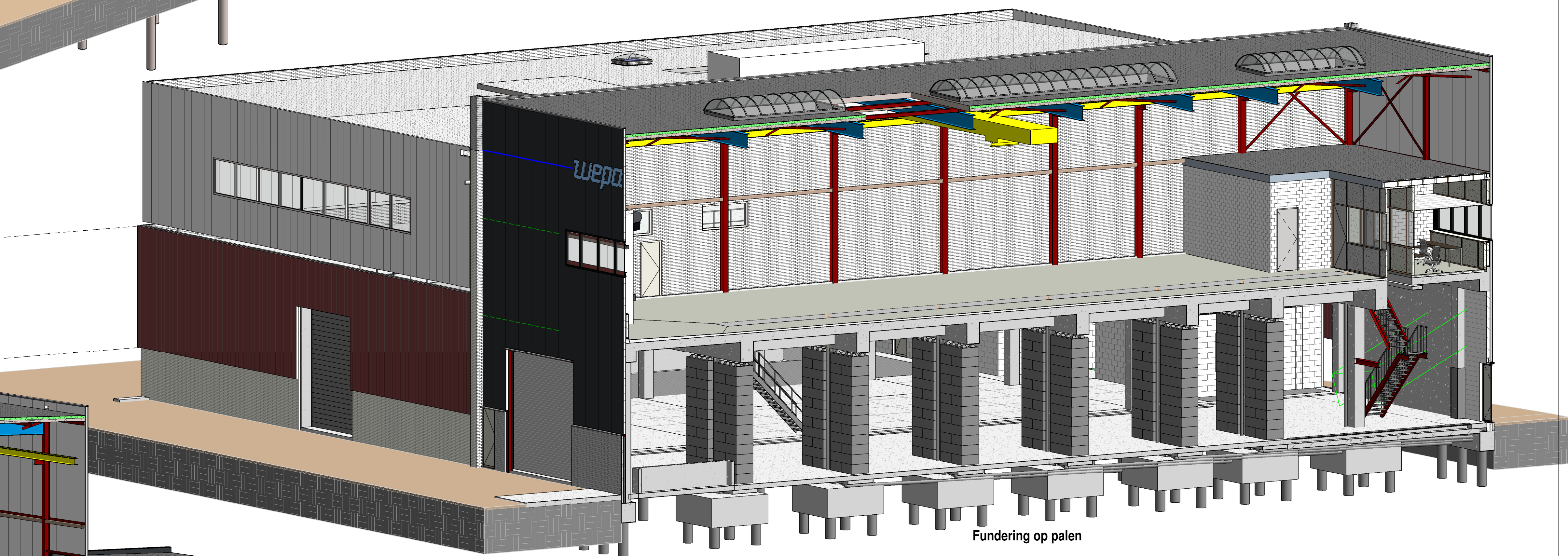
3D langsdoorsnede
