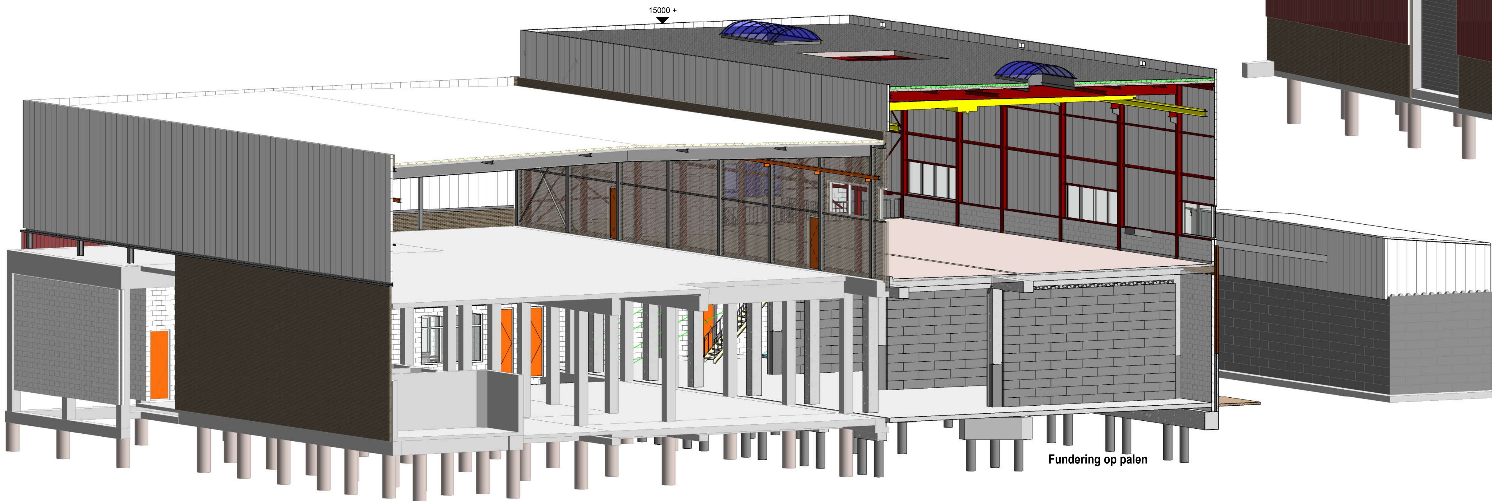
3D dwarsdoorsnede
