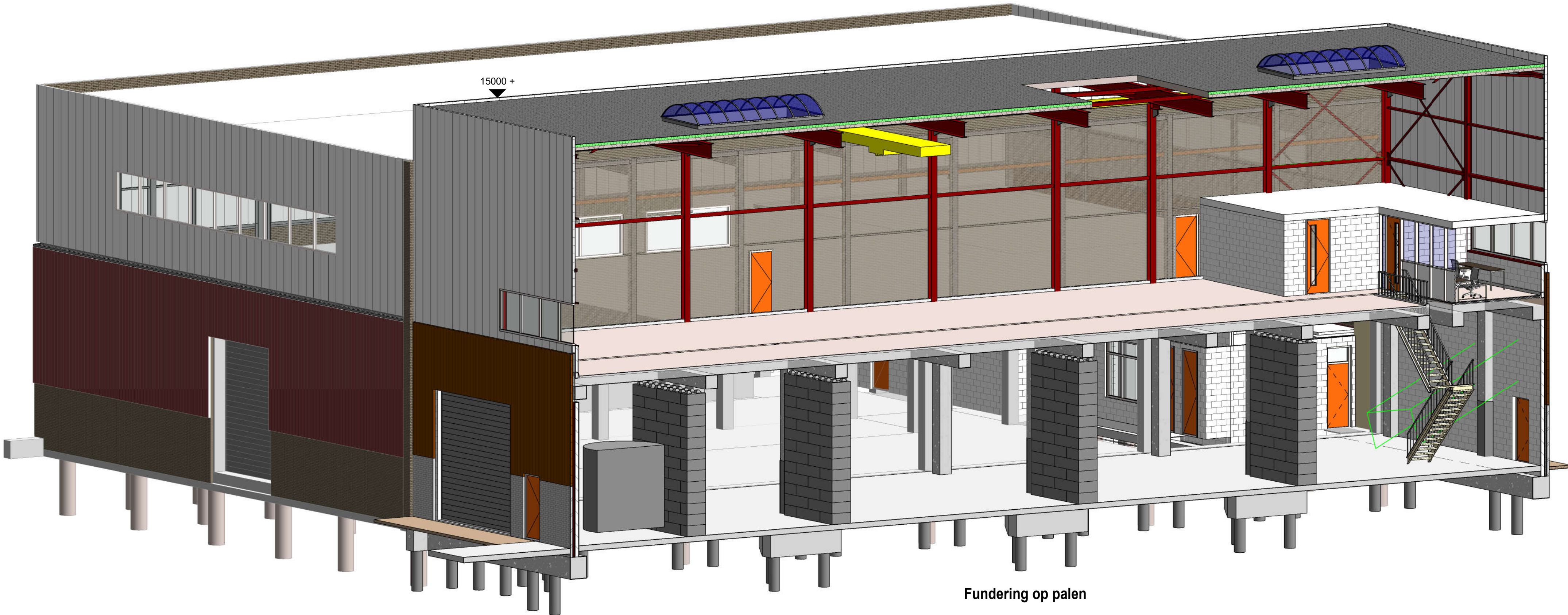
3D langsdoorsnede
