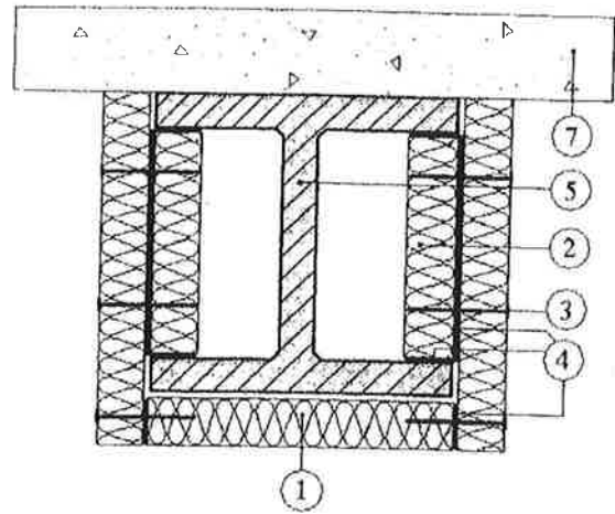
1b): Three-sided insulation
