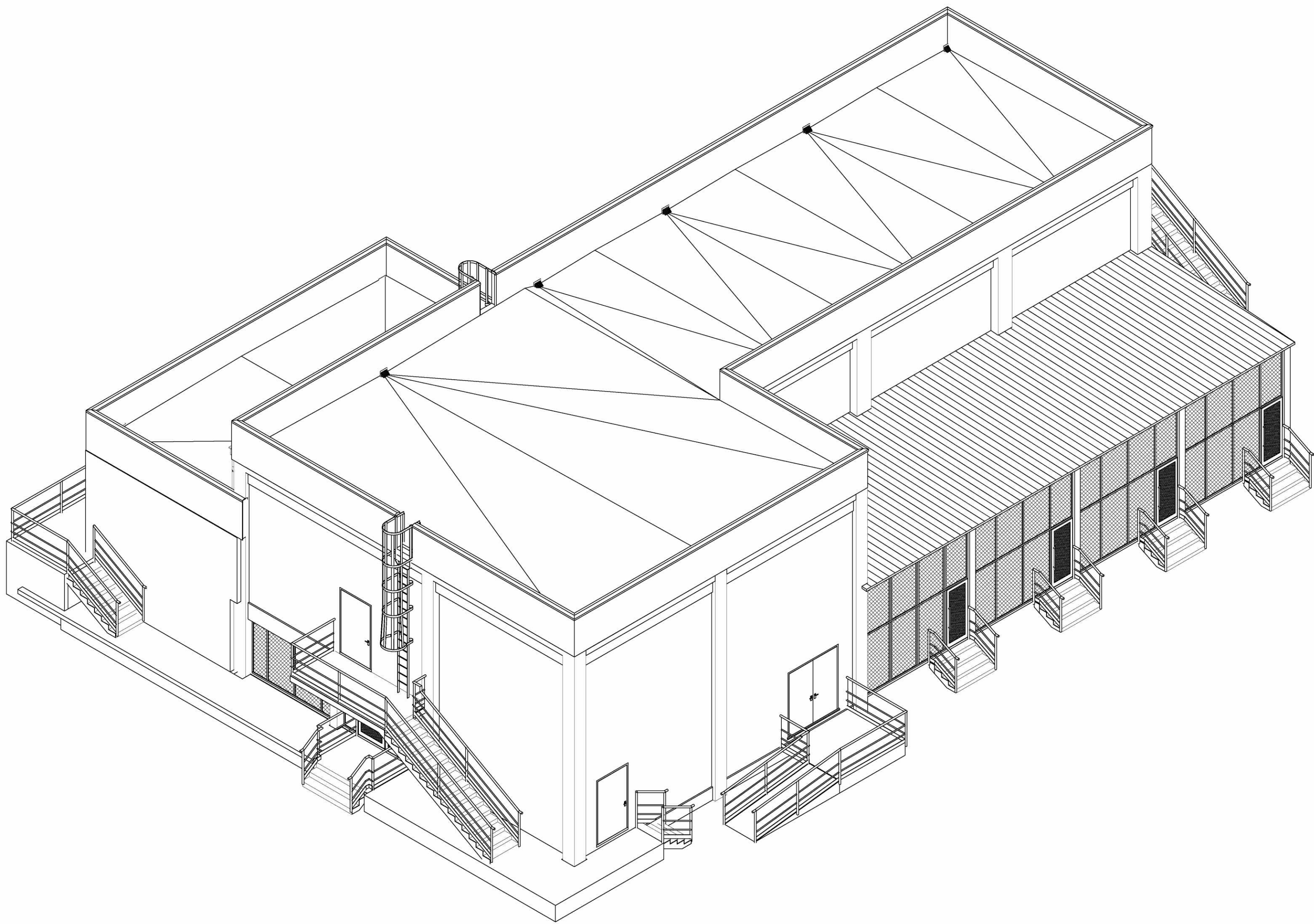
2 SOUTH-EAST VIEW 1 : 100
