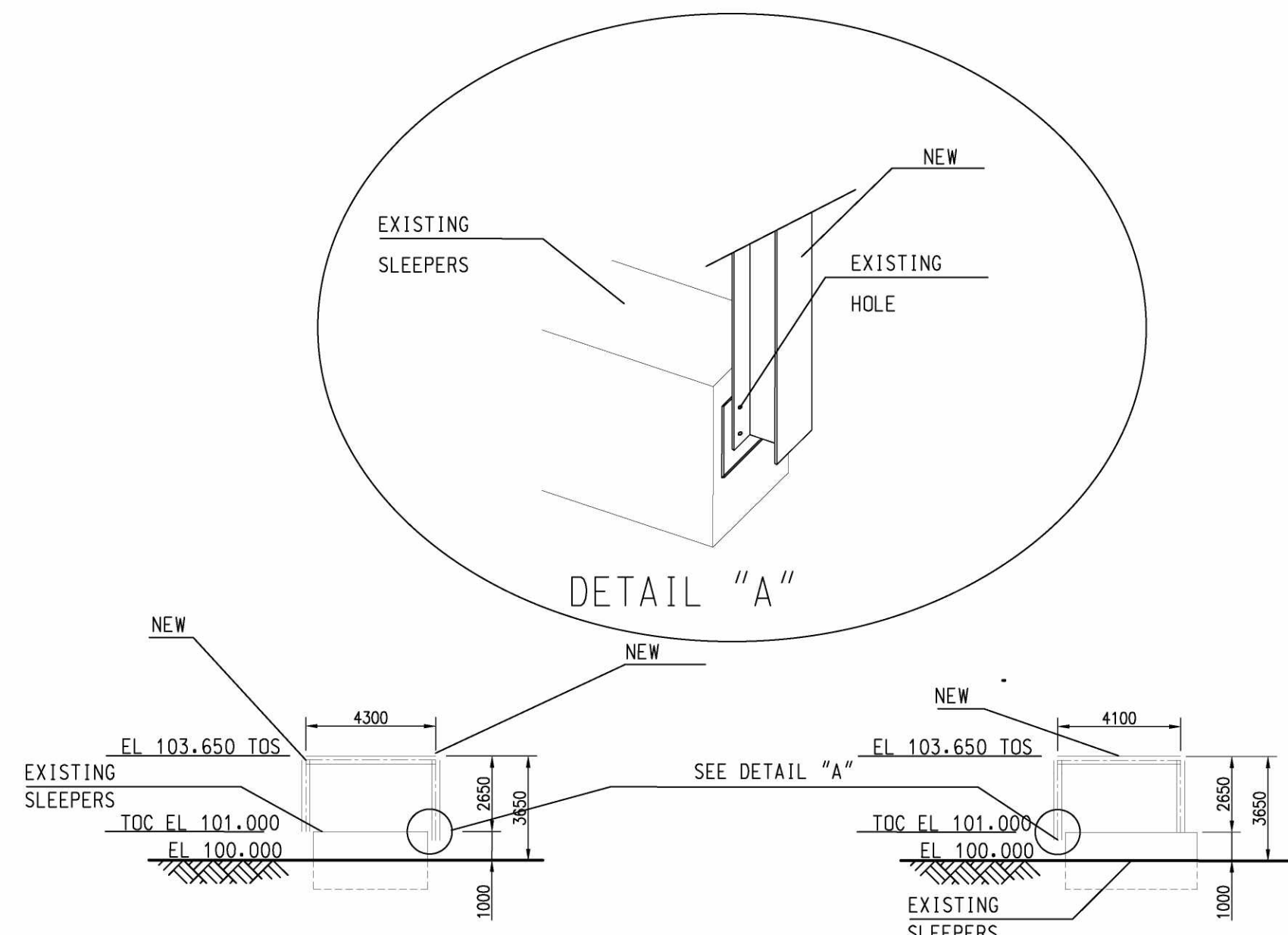
VIEW "D-D"
