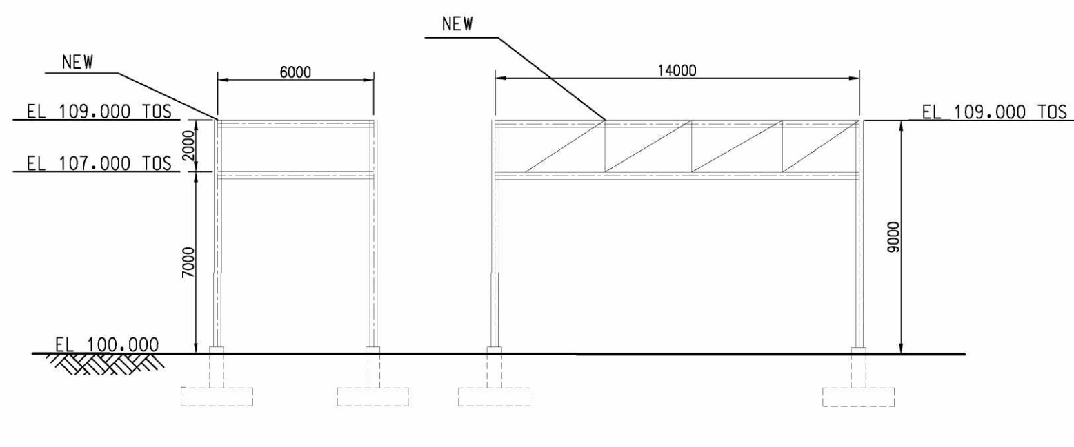
VIEW "I-I"
