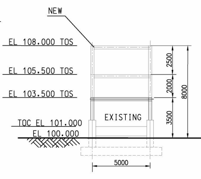
VIEW "M-M"
