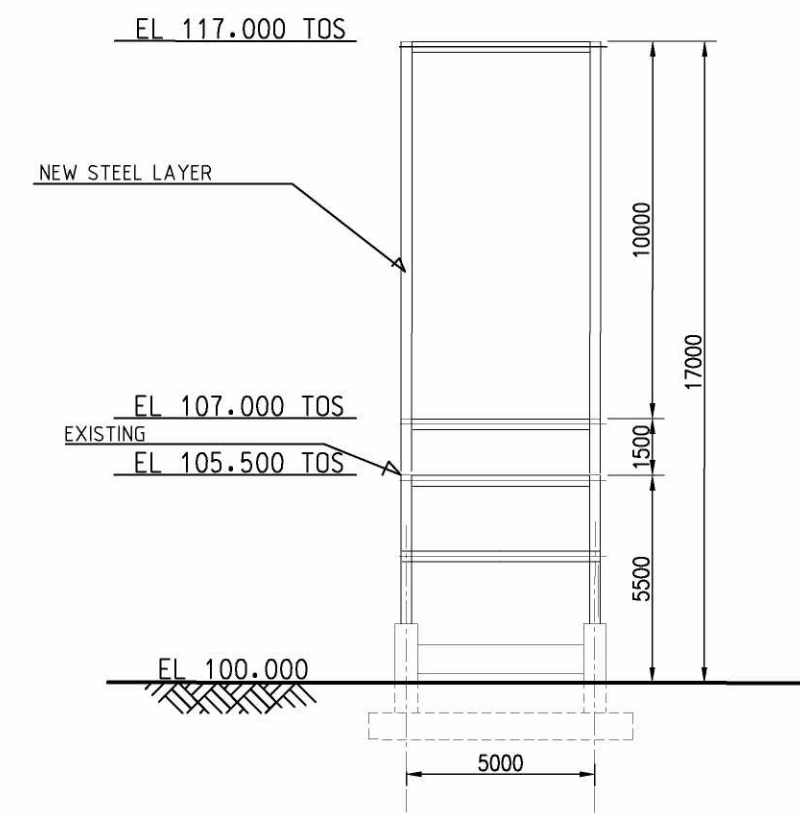
VIEW "Q-Q"
