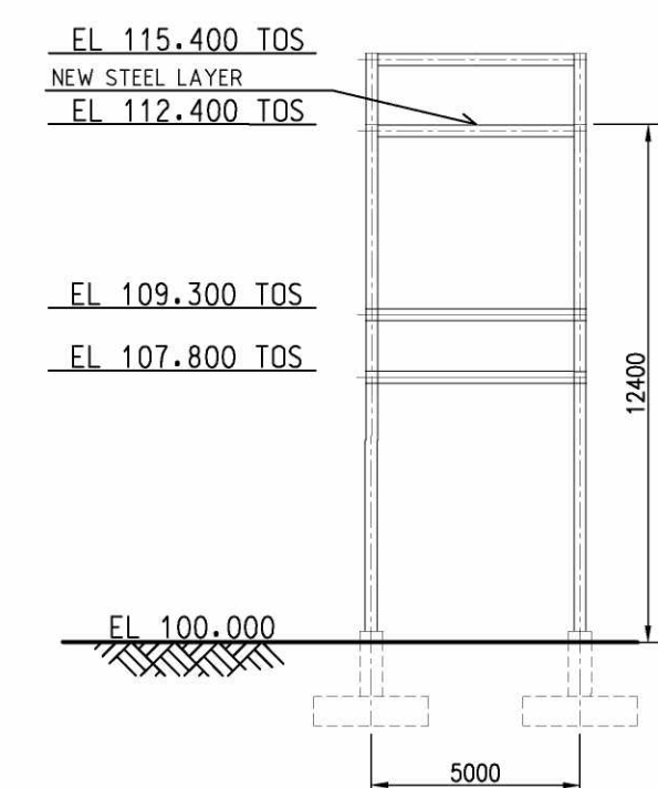
VIEW "R-R"
