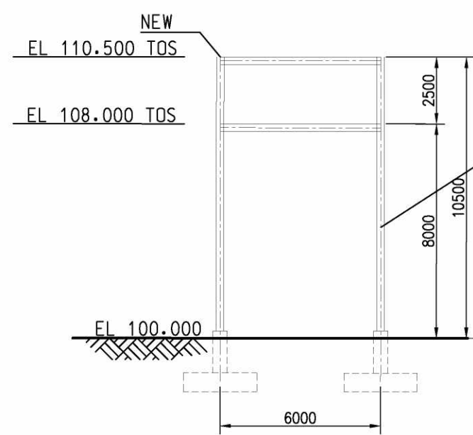
VIEW "F-F"
