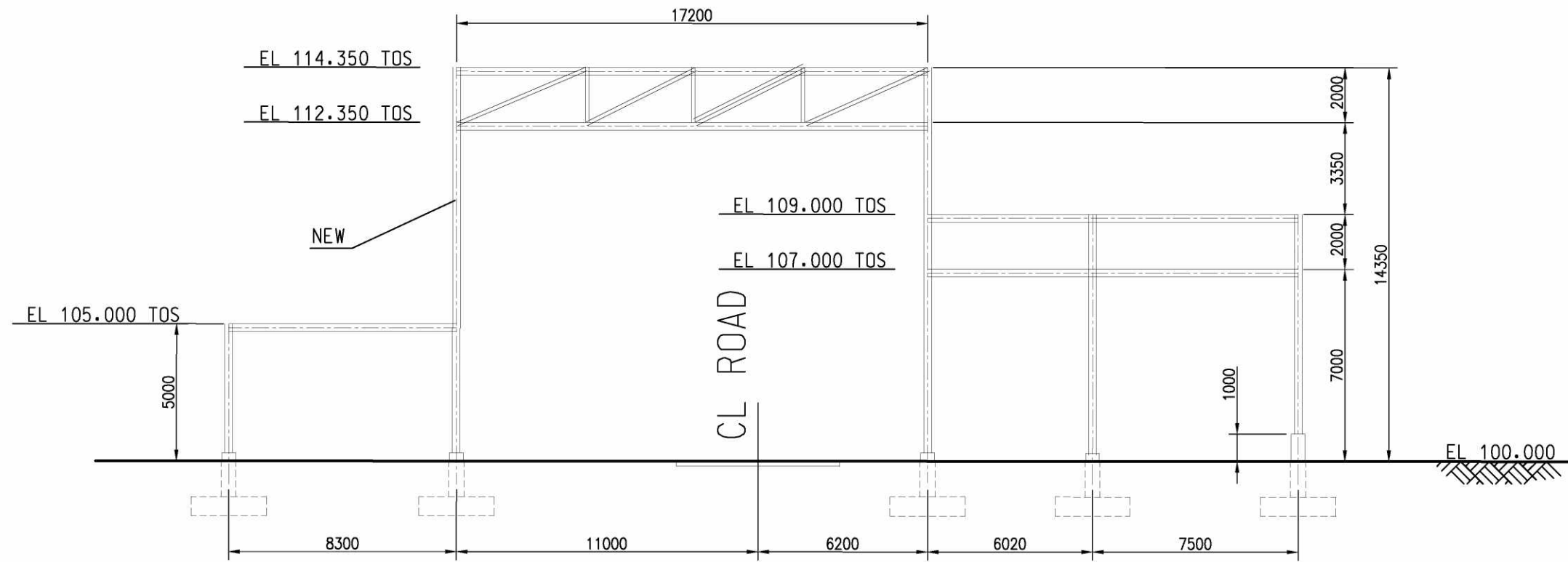
VIEW "C-C"
