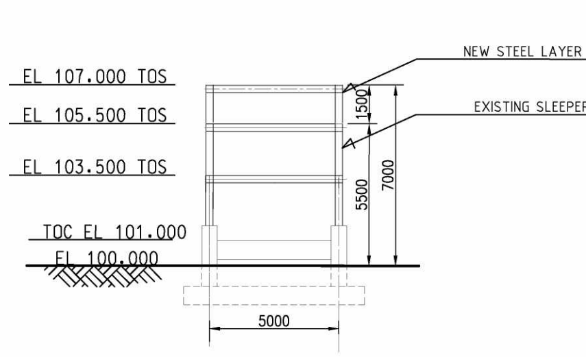
VIEW "P-P"
