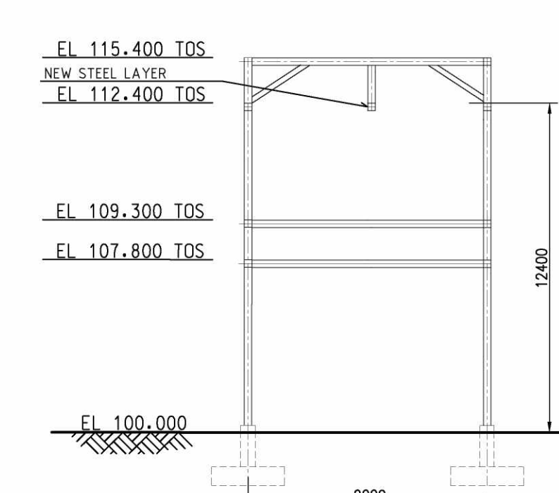
VIEW "R1-R1"
