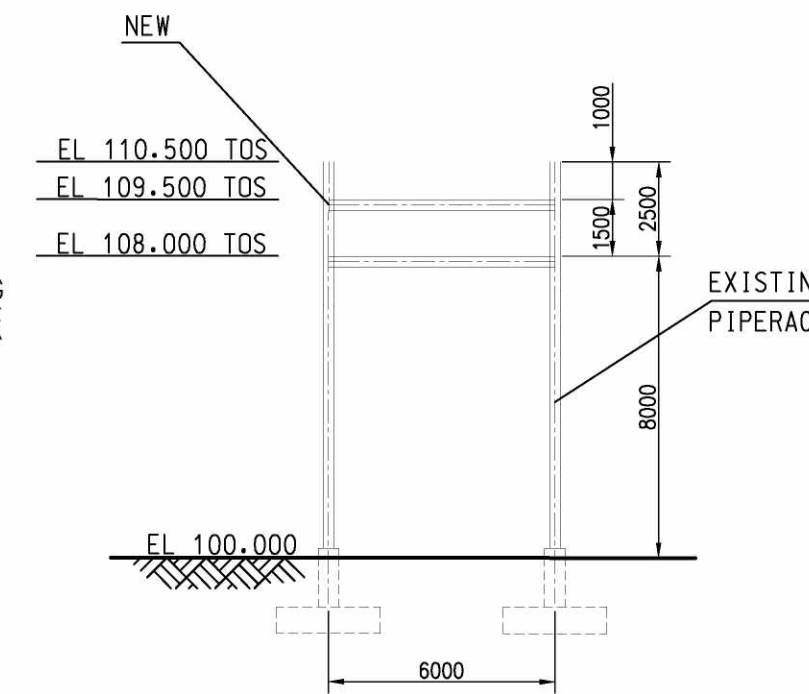
VIEW "G-G"
