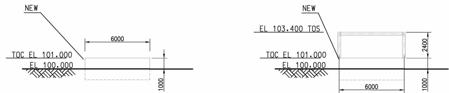
VIEW "A-A"
