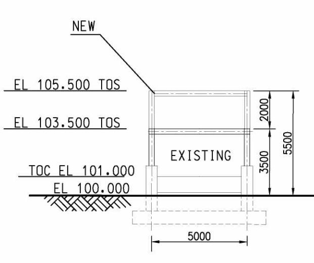
VIEW "O-O"
