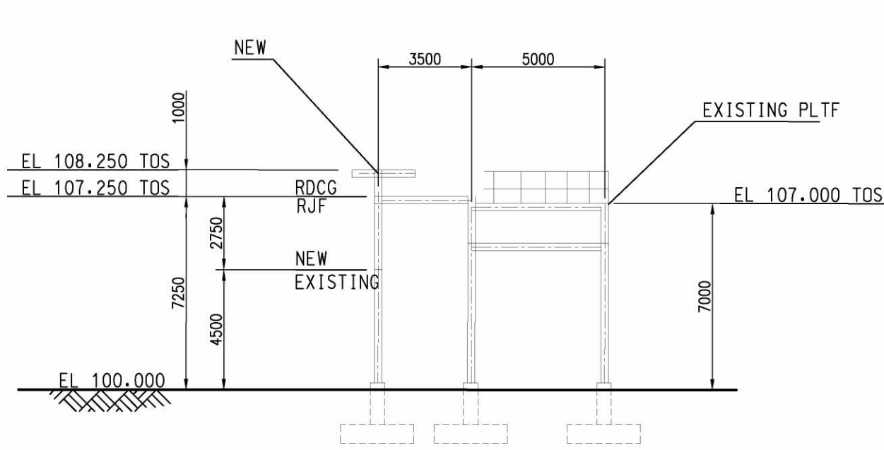
VIEW "T-T"
