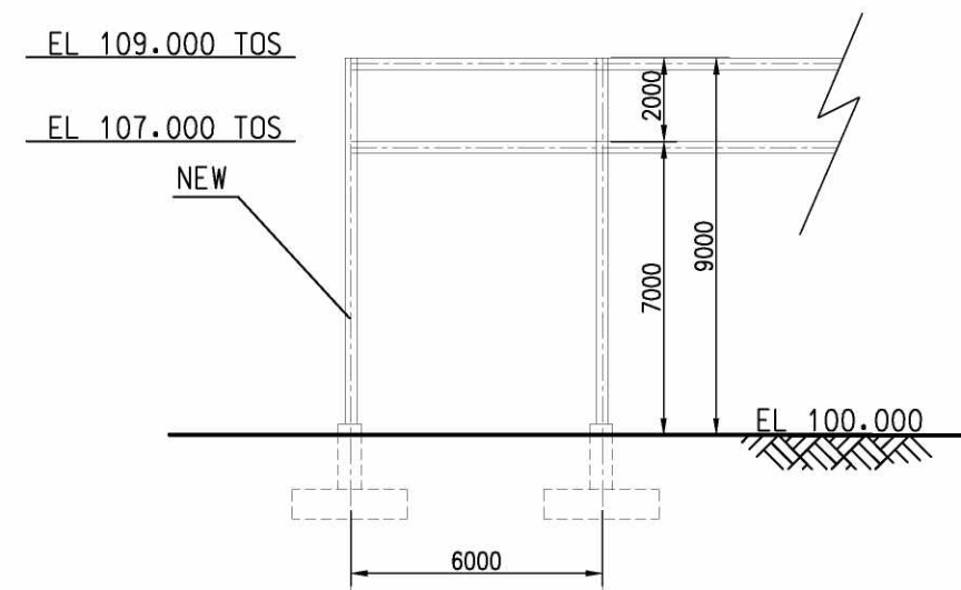
VIEW "B1-B1"
