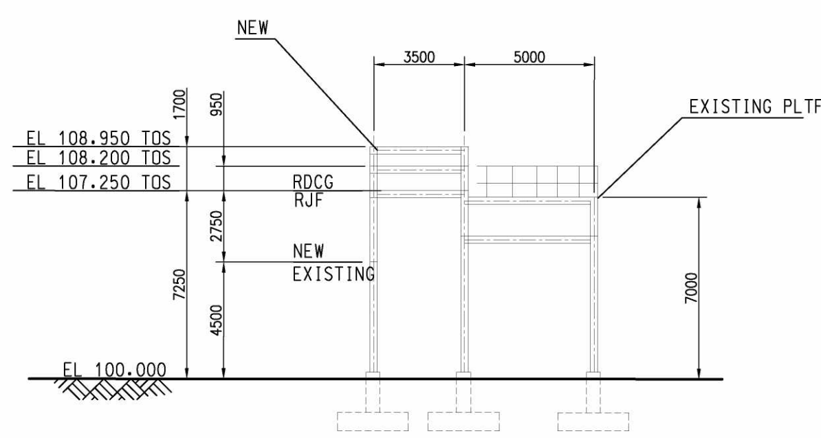
VIEW "S-S"
