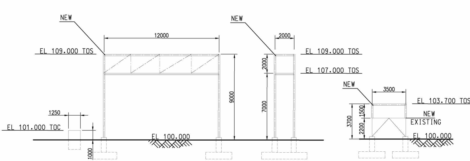
VIEW "Z-Z"
