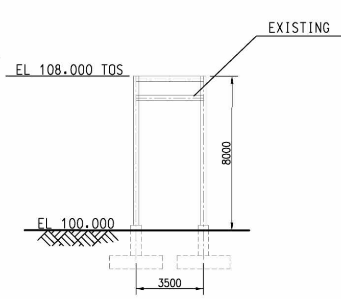
VIEW "L-L"
