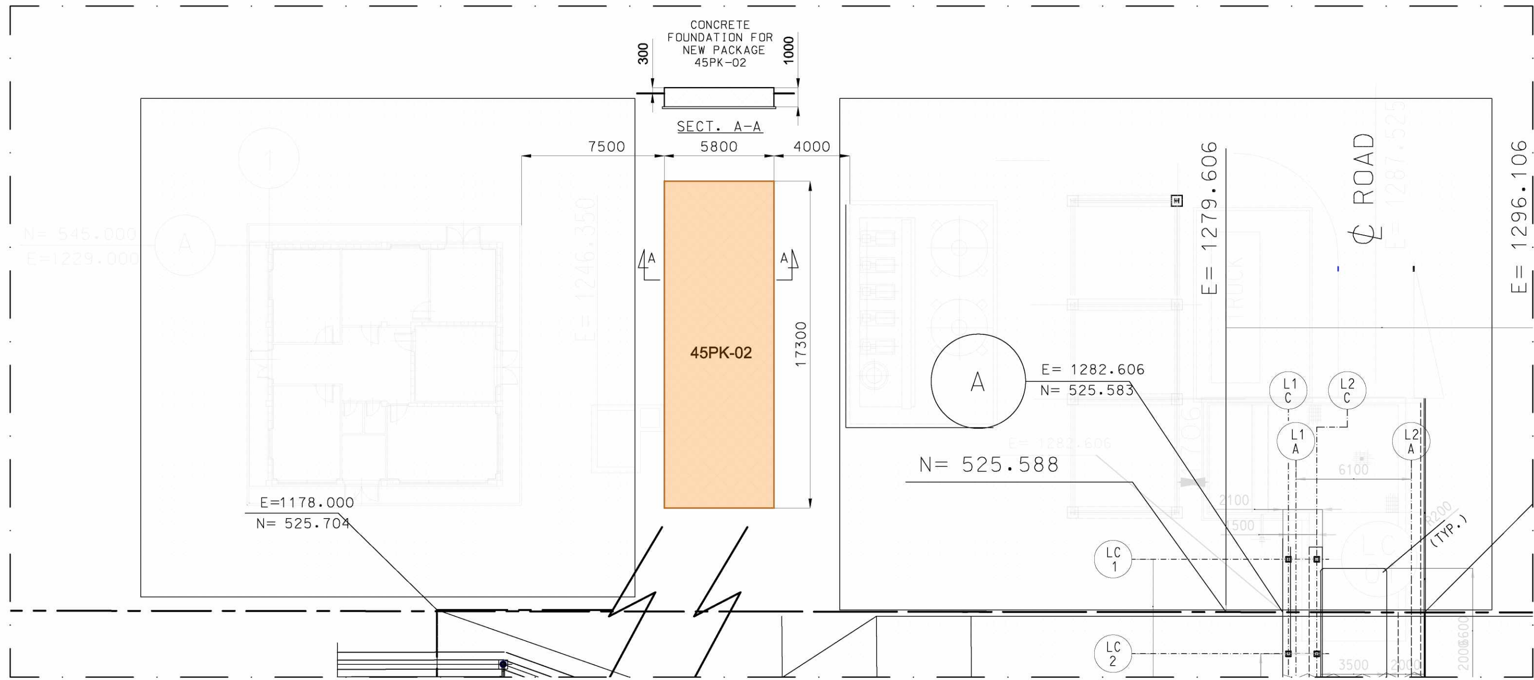
PLAN 1 (SCALE 1:200)
