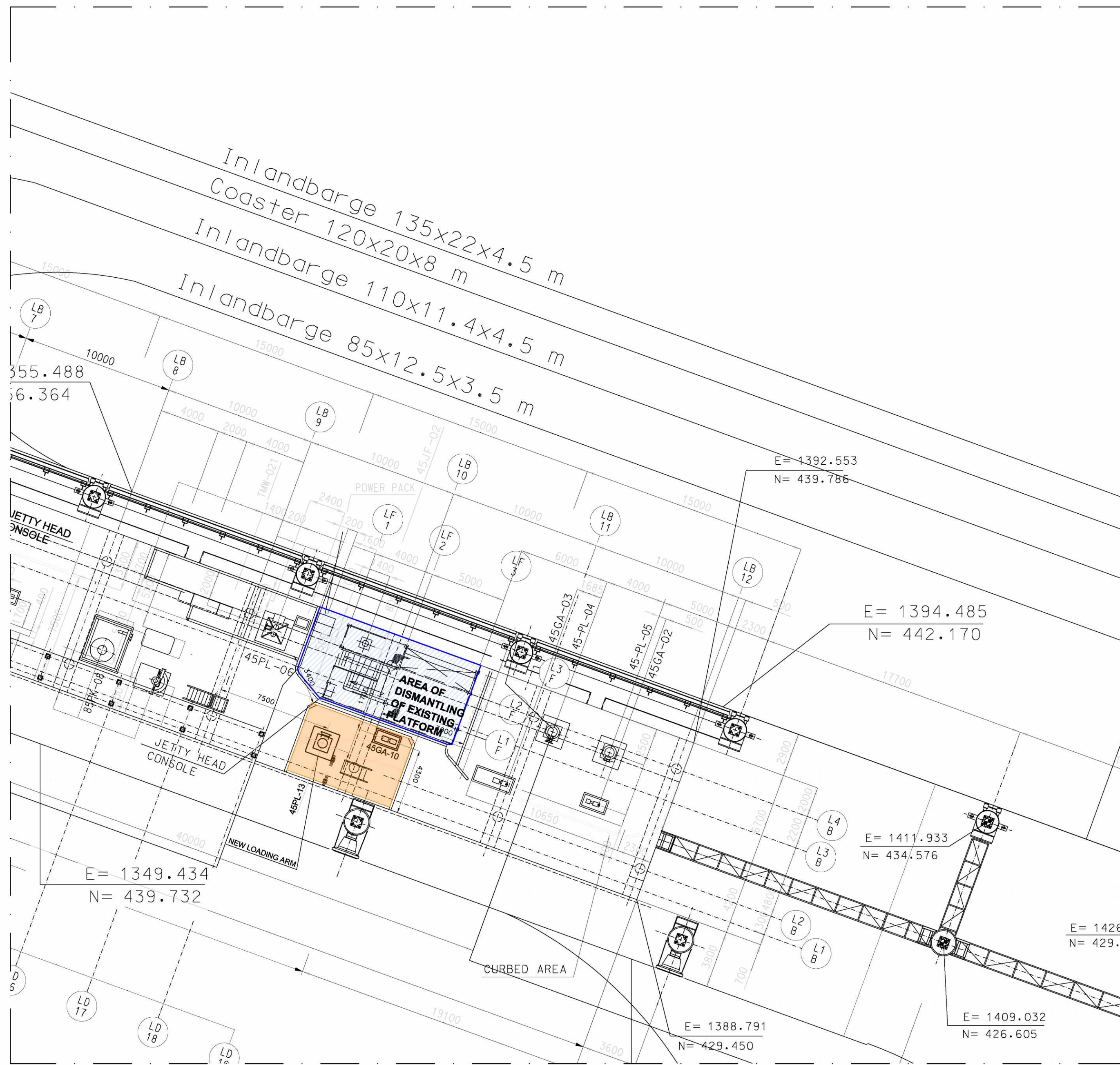
PLAN 2 (SCALE 1:200)
