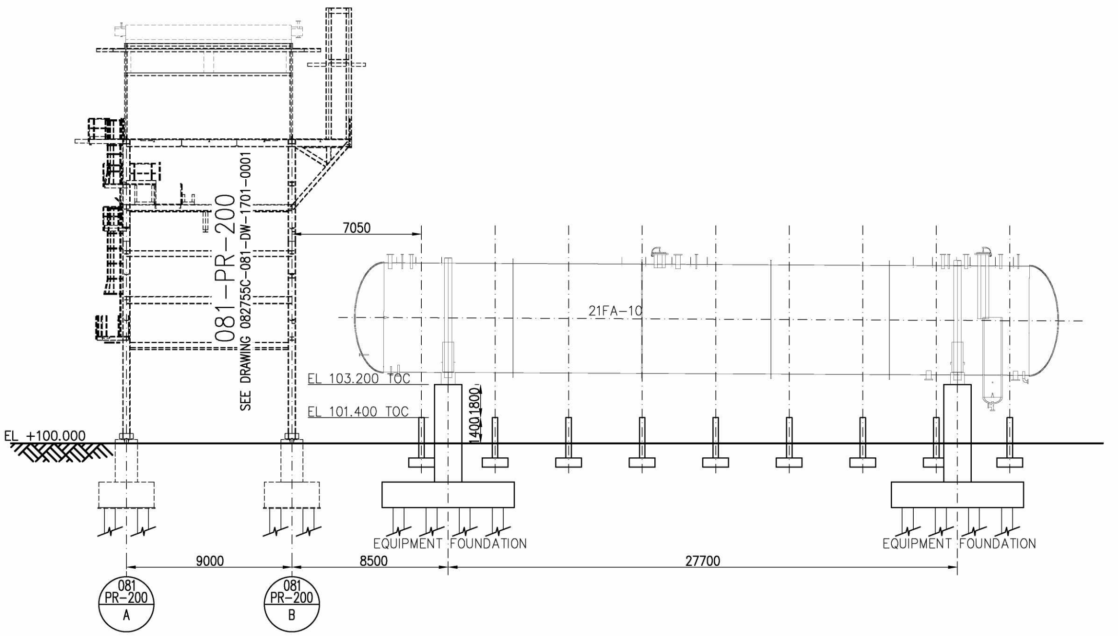
VIEW "N-N"
