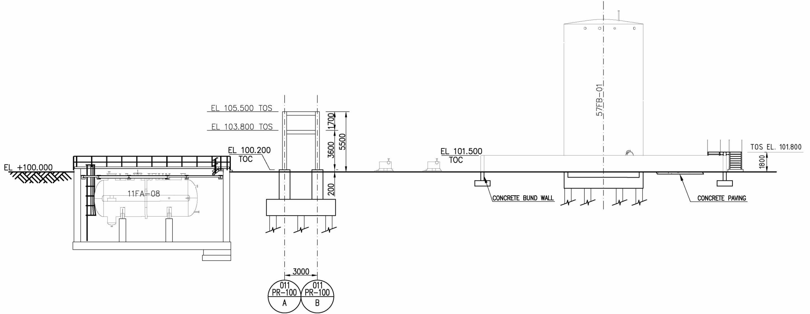
VIEW "M-M"
