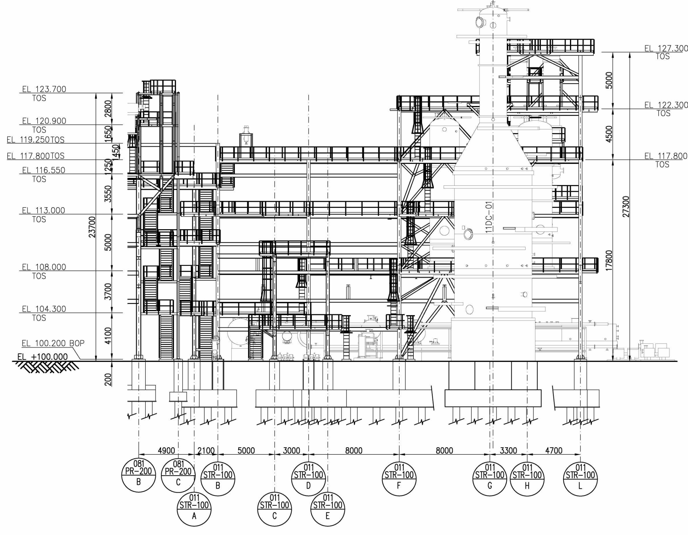
057-STIR-100 VIEW "L-L"
