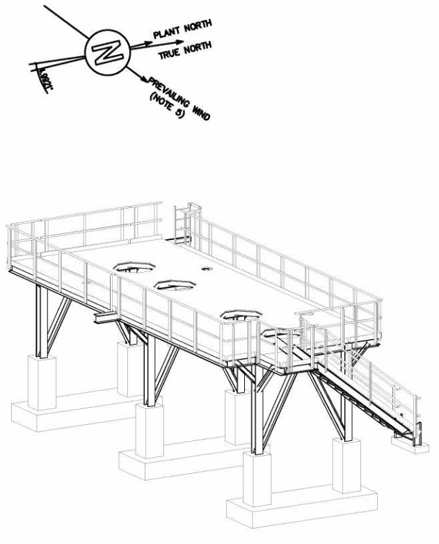
021-STR-1000 ISOMETRIC VIEW "1"
