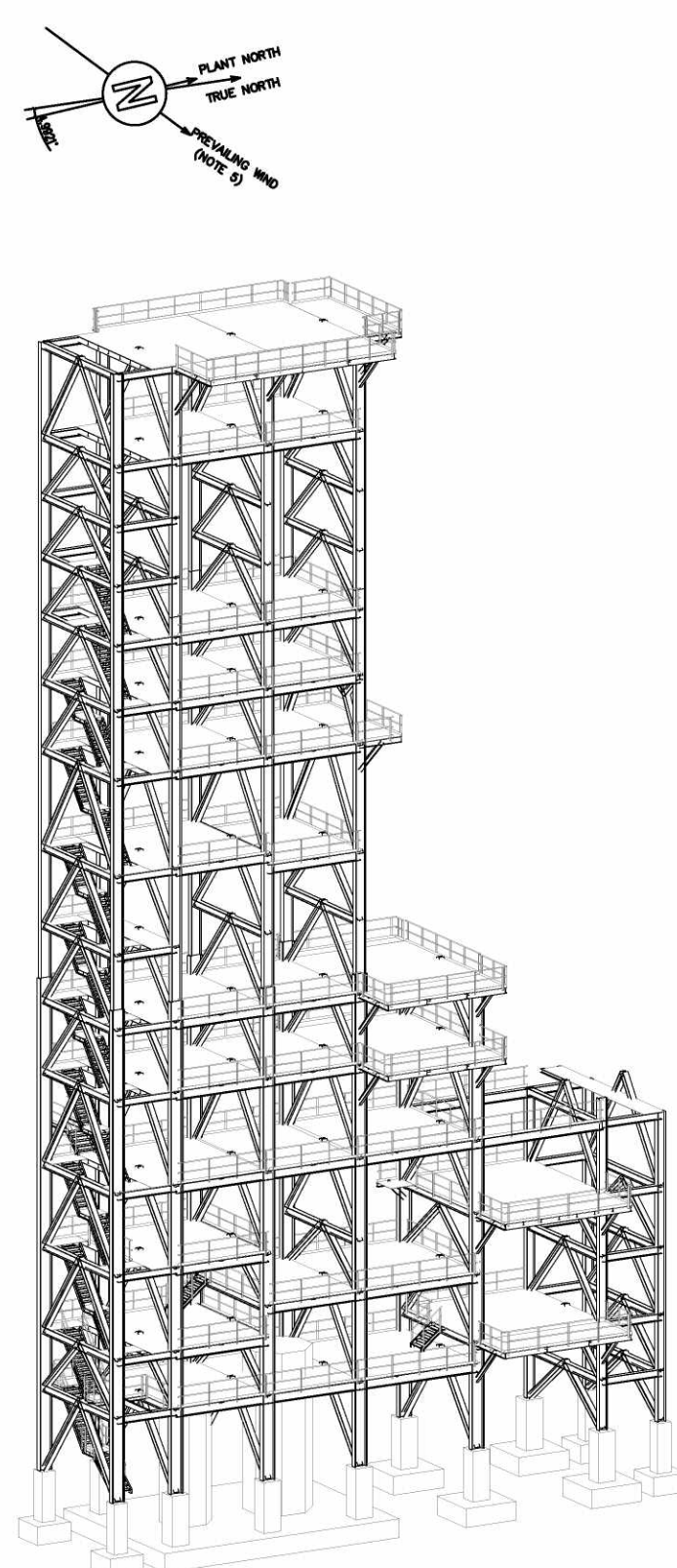
021-STR-1200 ISOMETRIC VIEW "1"
