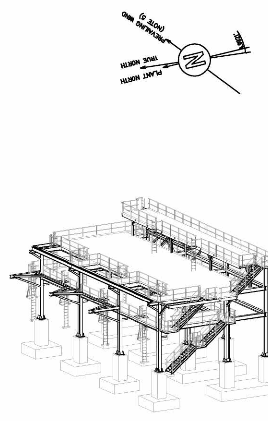
021-STR-600 ISOMETRIC VIEW "2"
