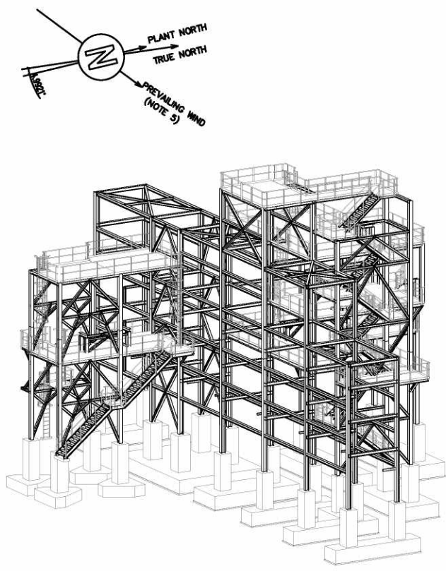
021-STR-400 ISOMETRIC VIEW "1"
