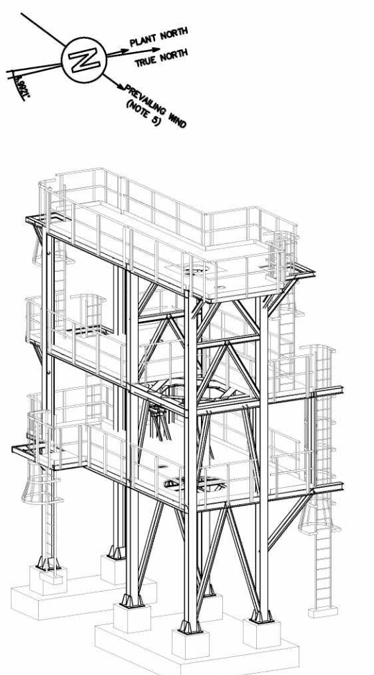
021-STR-1100 ISOMETRIC VIEW "1"
