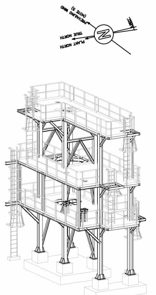
021-STR-1100 ISOMETRIC VIEW "2"
