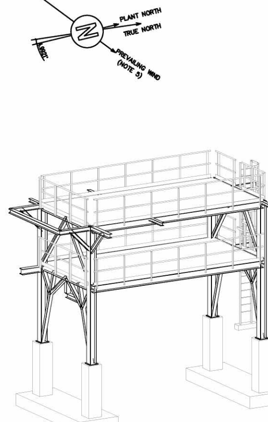
021-PLT-101 ISOMETRIC VIEW "1"
