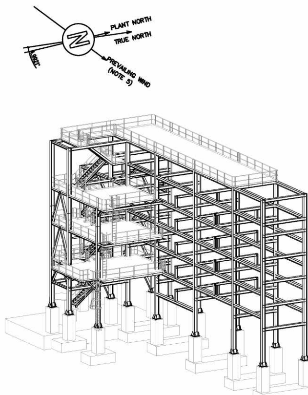
021-STR-500 ISOMETRIC VIEW "1"
