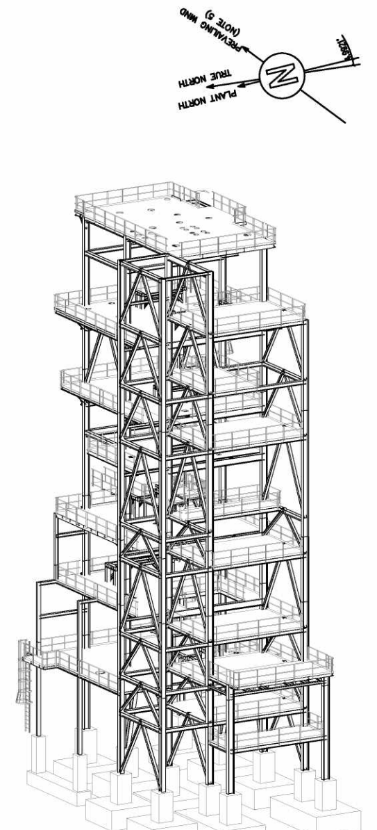
021-STR-900 ISOMETRIC VIEW "2"
