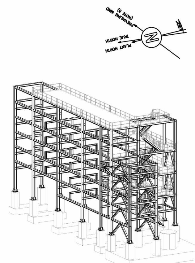
021-STR-500 ISOMETRIC VIEW "2"
