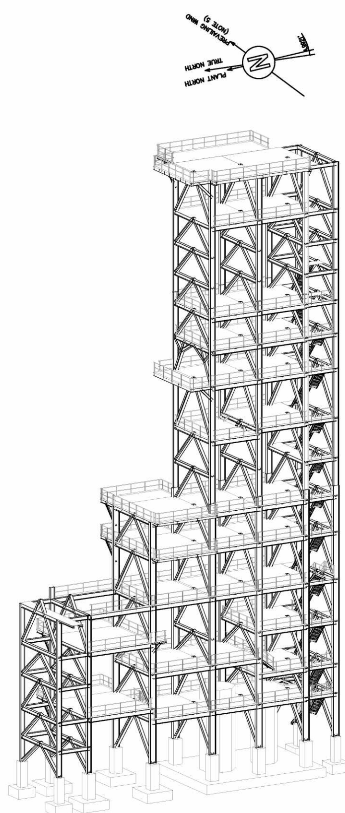
021-STR-1200 ISOMETRIC VIEW "2"
