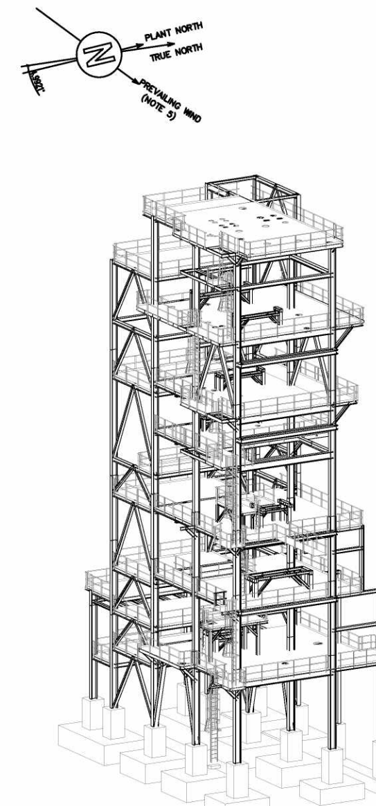
021-STR-900 ISOMETRIC VIEW "1"
