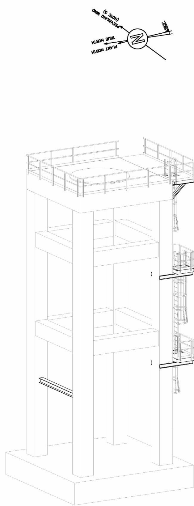
021-STR-1300 ISOMETRIC VIEW "2"
