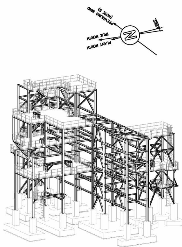
021-STR-400 ISOMETRIC VIEW "2"
