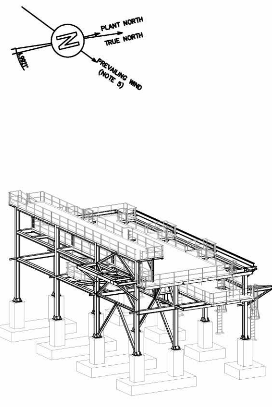
021-STR-600 ISOMETRIC VIEW "1"
