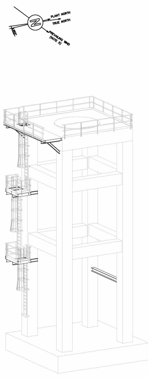
021-STR-1300 ISOMETRIC VIEW "1"
