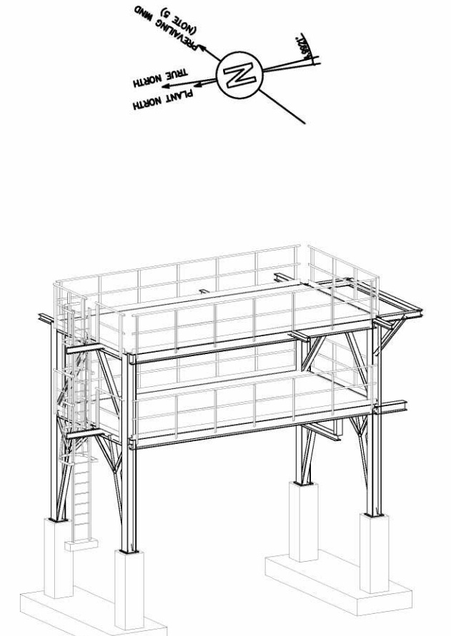
021-PLT-101 ISOMETRIC VIEW "2"
