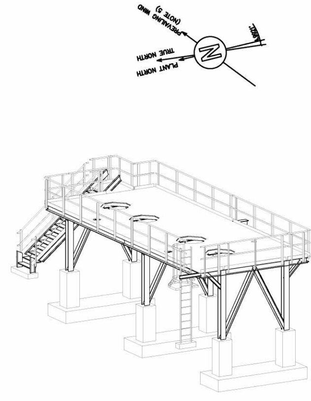
021-STR-1000 ISOMETRIC VIEW "2"
