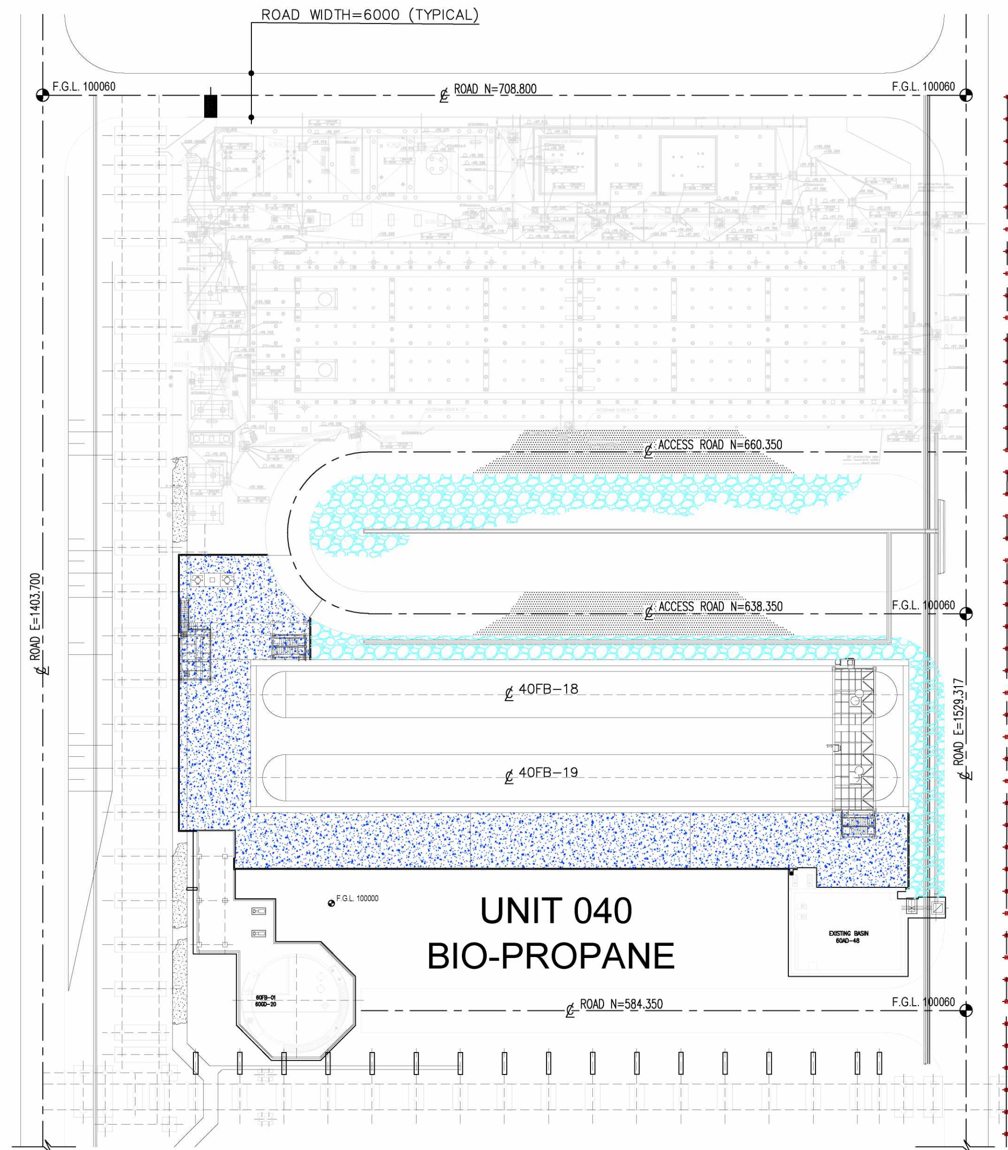
MAJOR LAYOUT AREA ③
