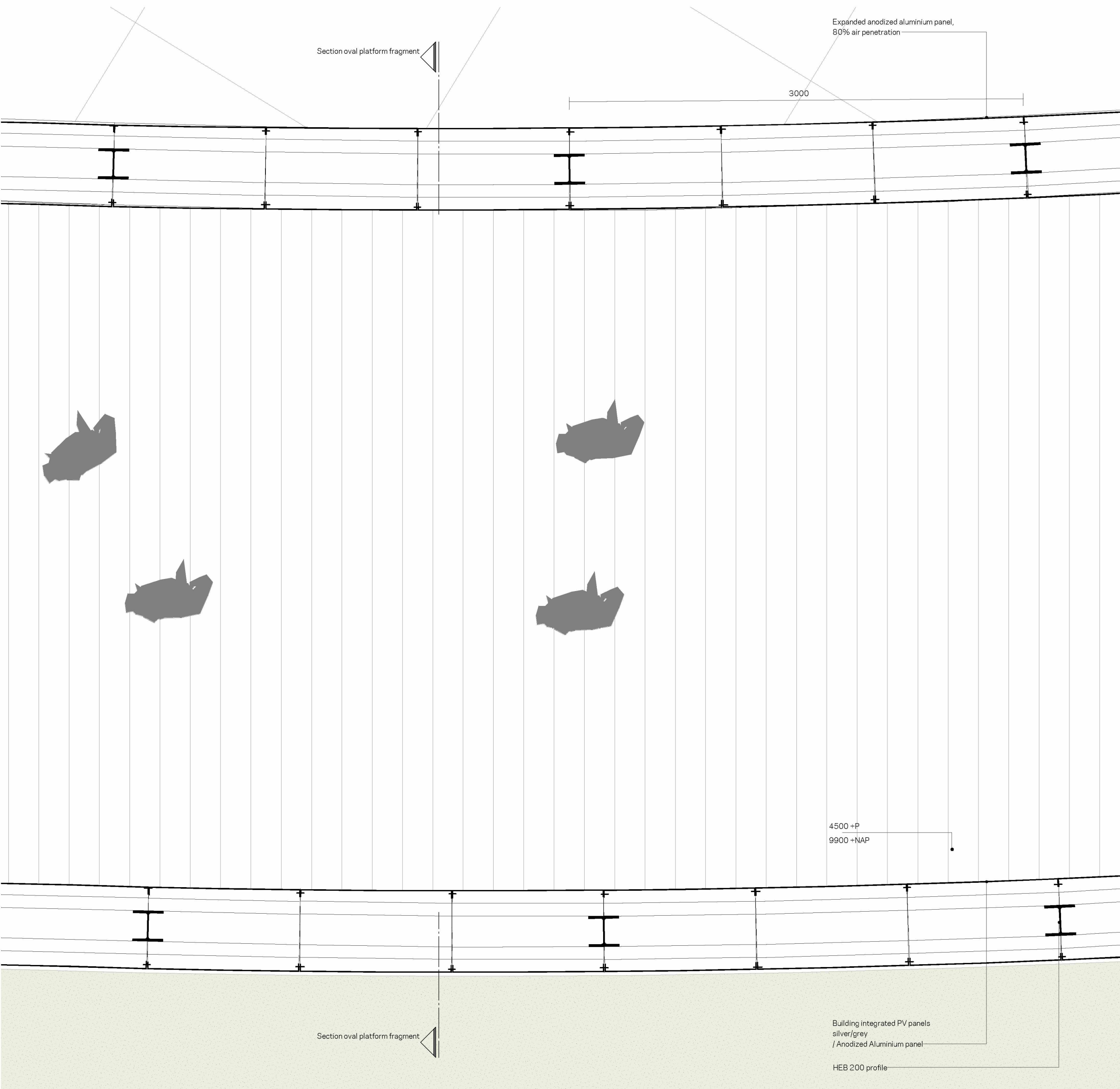
Floorplan oval fragment
