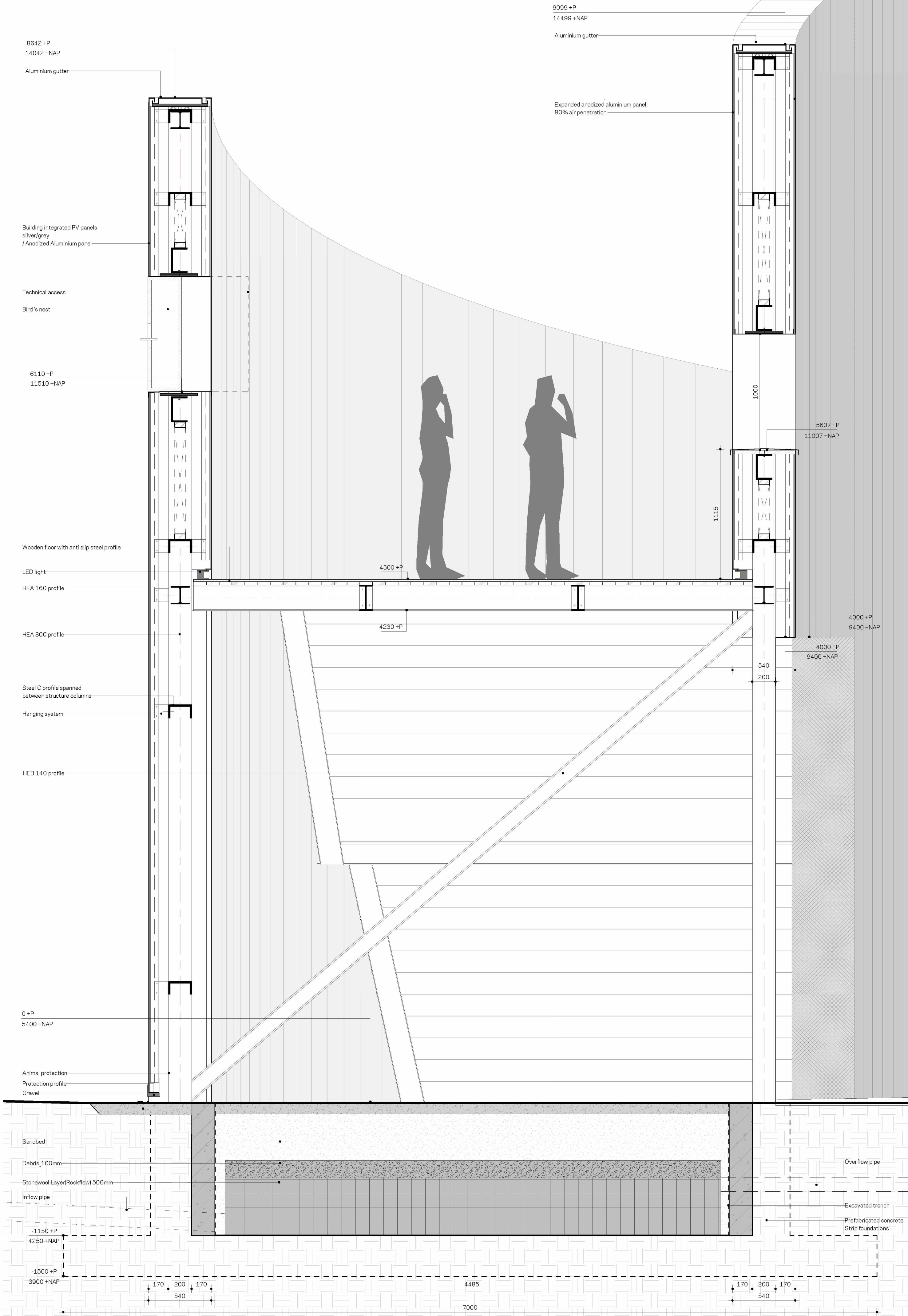
Section oval fragment
