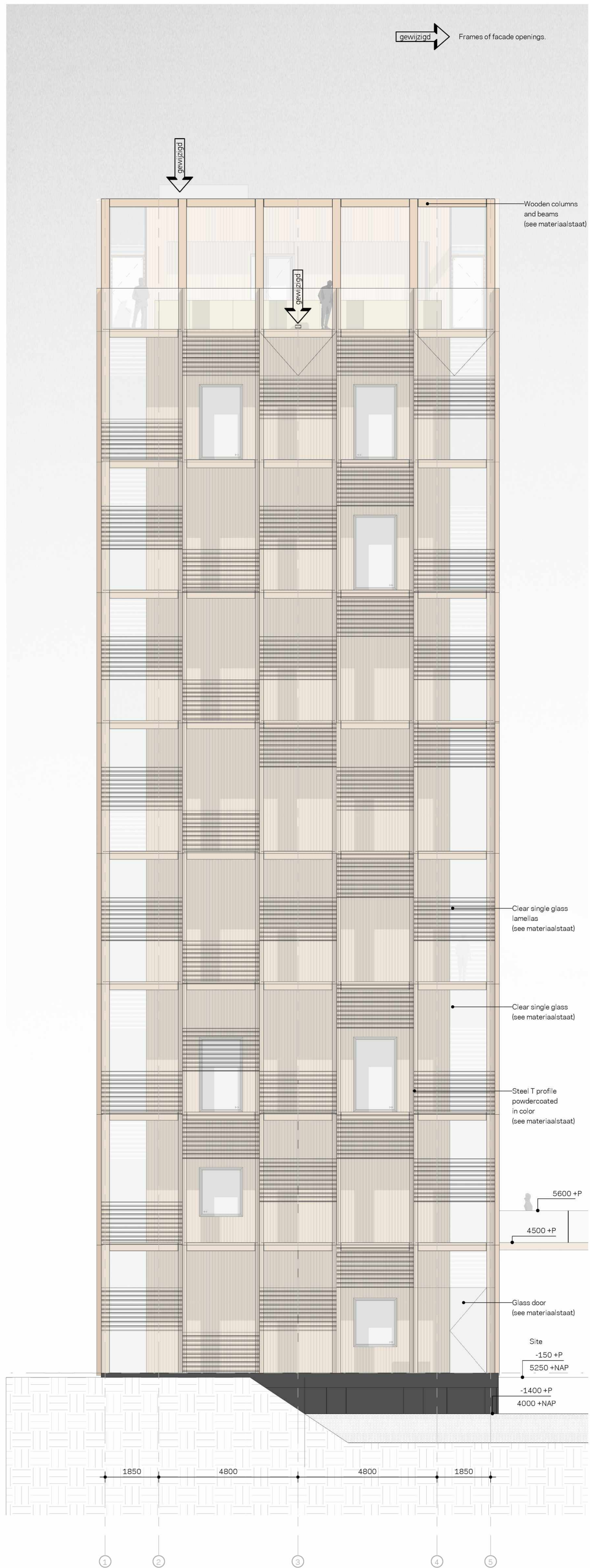
West elevation
