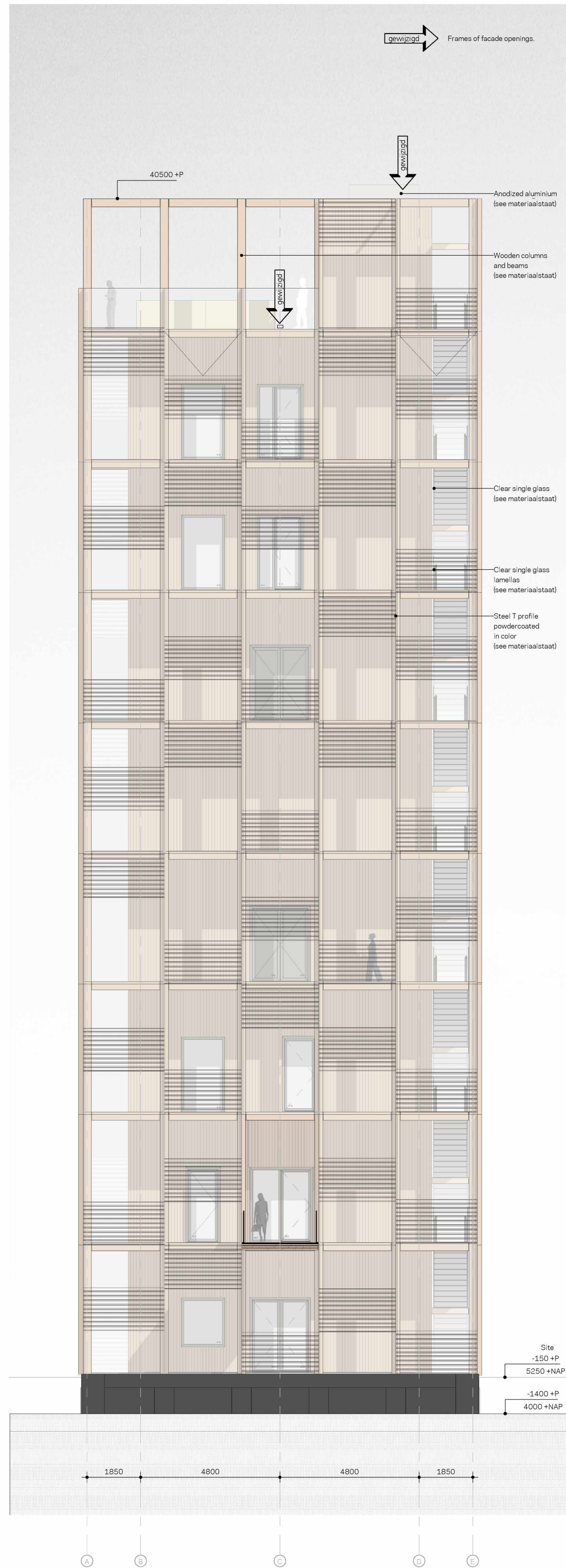
South elevation
