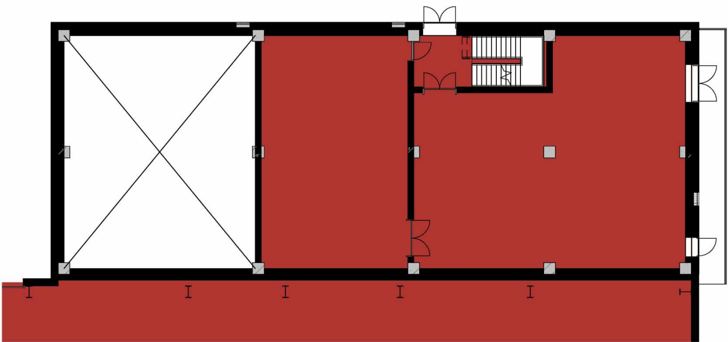
Annex building first floor_IT
