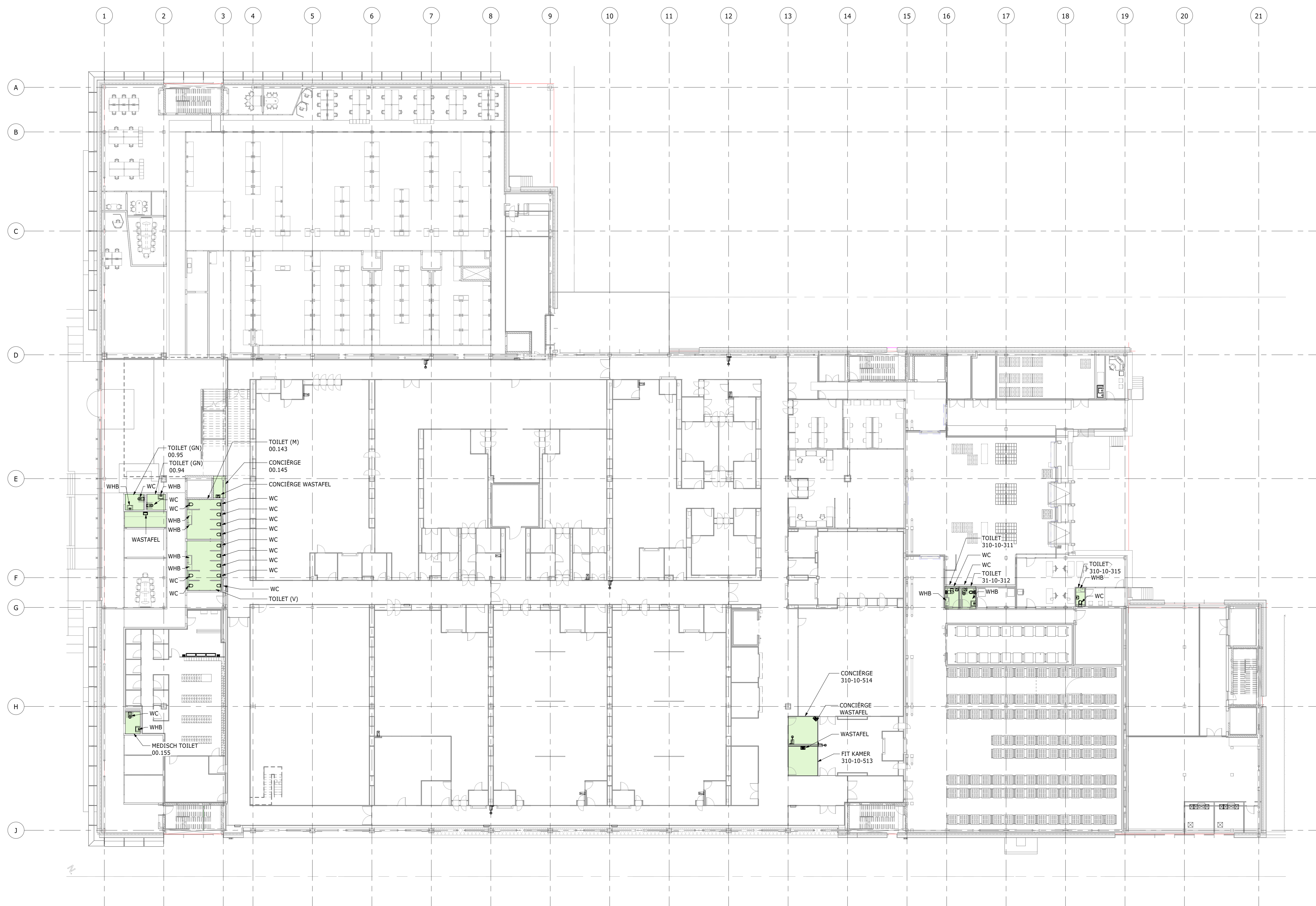
LEVEL 00 - DUTCH WATER OUTLETS GROUND FLOOR LAYOUT SCALE: 1 : 200
