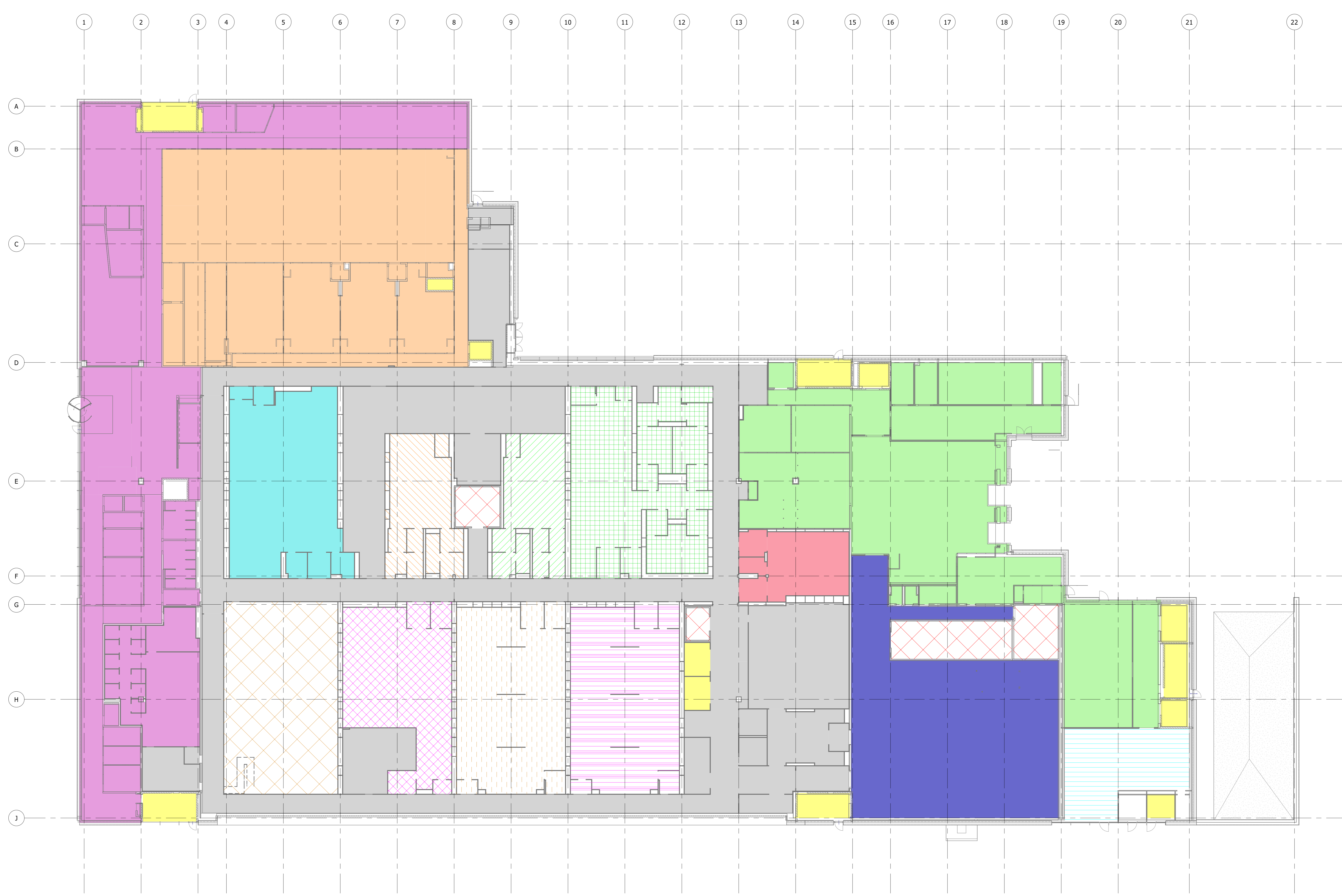
LEVEL 00 - AHU SYSTEM LAYOUT SCALE: 1 : 200
