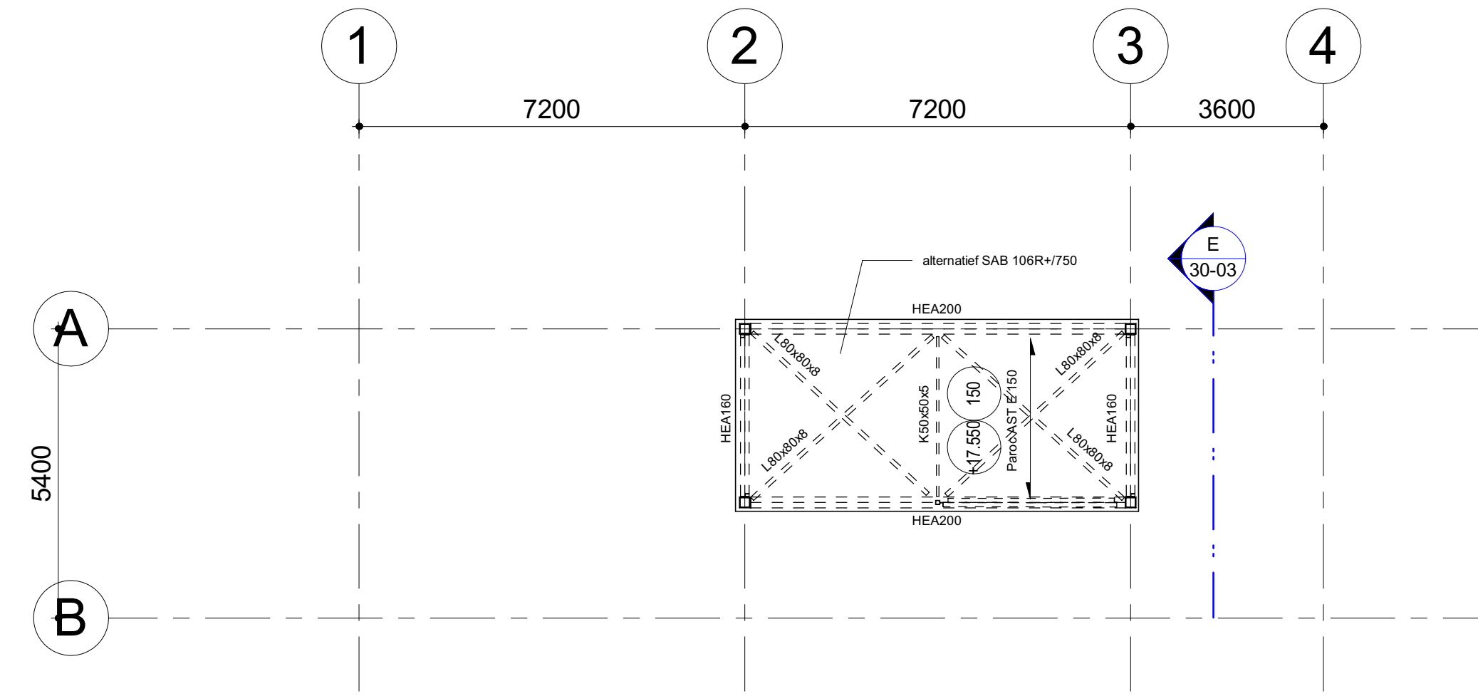
2 Dak trappenhuis as A / 2-3 Schaal: 1:100
