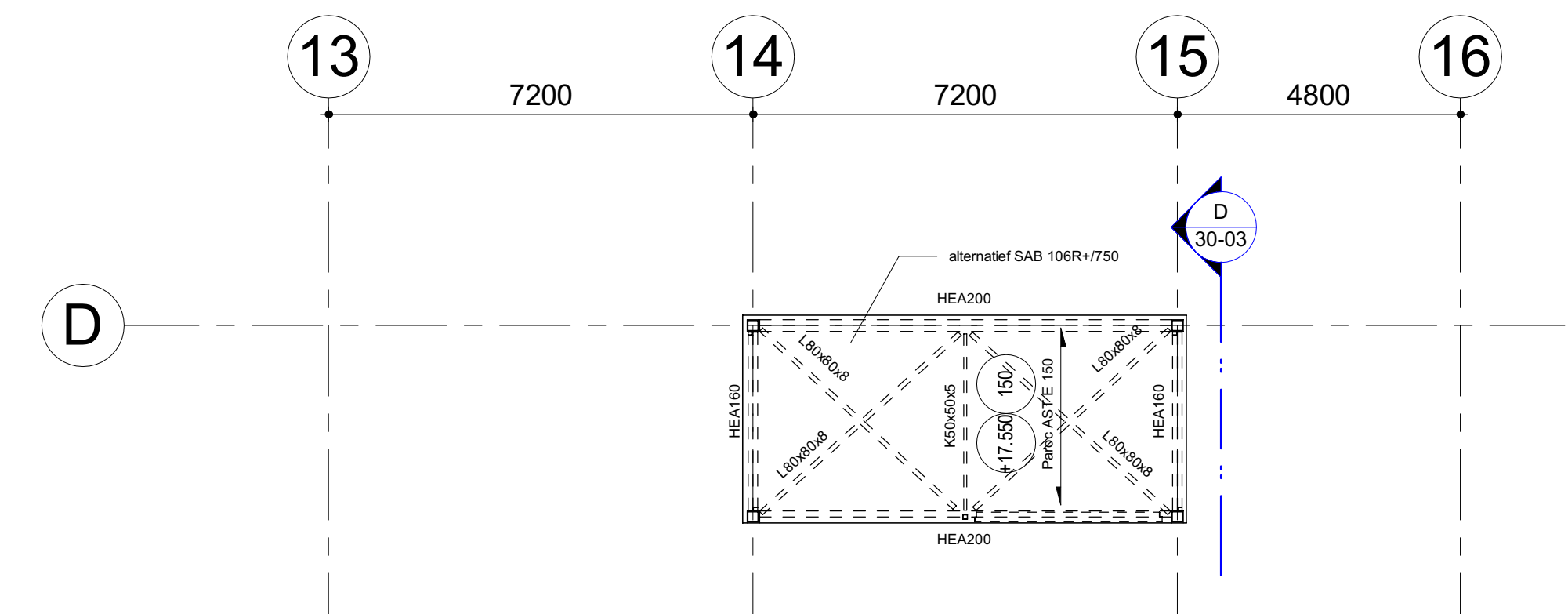
4 Dak trappenhuis as D / 14-15 Schaal: 1:100
