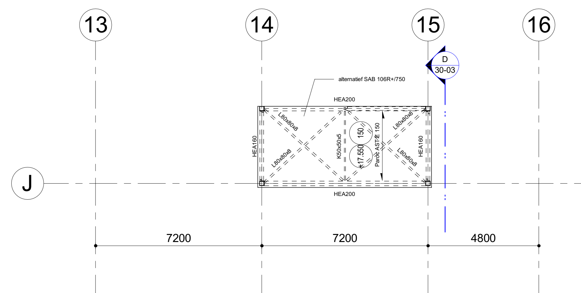
5 Dak trappenhuis as J / 14-15 Schaal: 1:100
